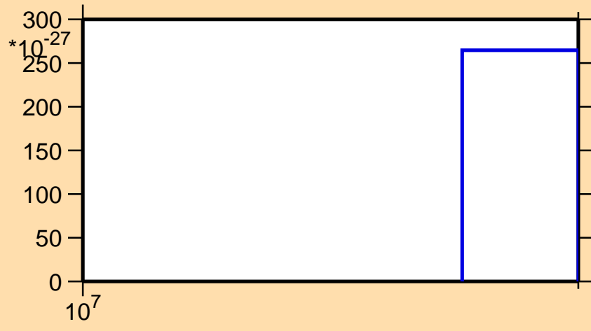
\sigma vs. E for ^{151}\text{Pr}(\text{mt } 42)
