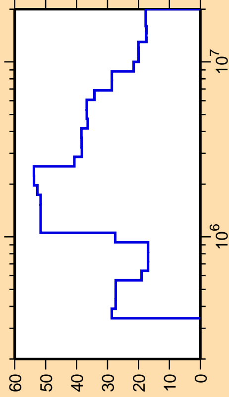
\Delta\sigma/\sigma vs. E for ^{151}\text{Pr}(n,n_3)
