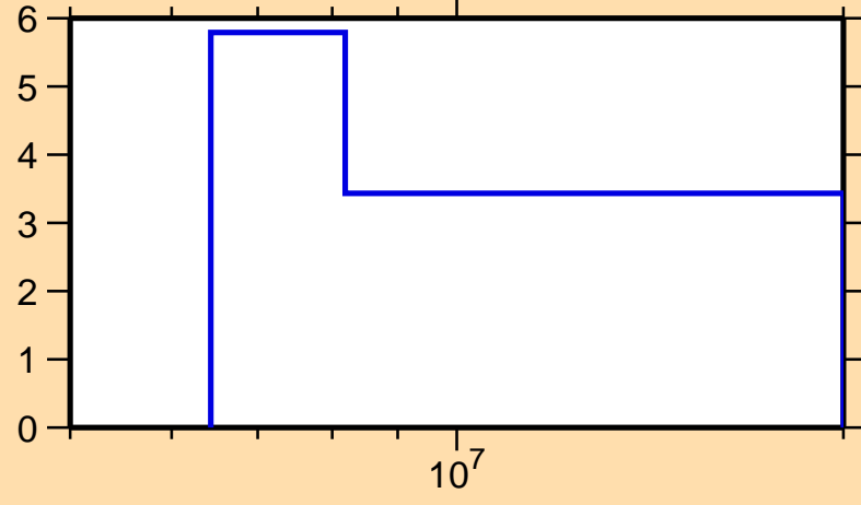
\Delta\sigma/\sigma vs. E for ^{151}\text{Pr}(n,\text{tot.})
