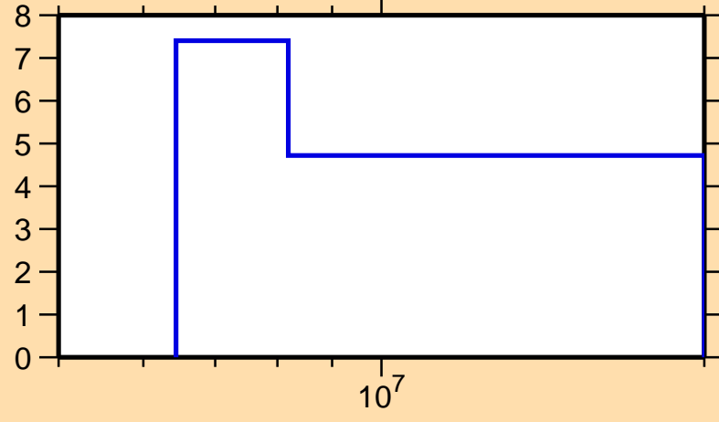
\Delta\sigma/\sigma vs. E for ^{151}\text{Pr}(n,\text{el.})
