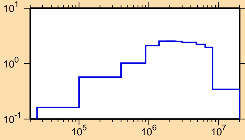
\sigma vs. E for ^{151}\text{Pr}(n,\text{inel.})
