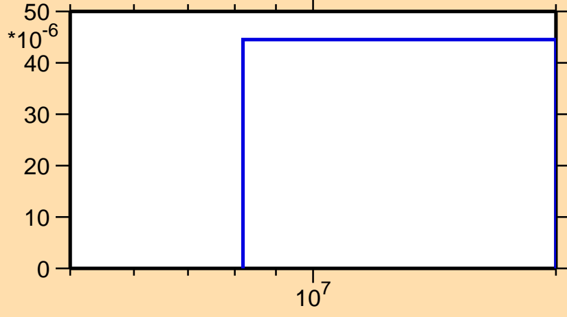
\sigma vs. E for ^{151}\text{Pr}(n,d)
