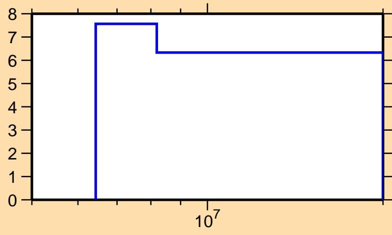
\Delta\sigma/\sigma vs. E for ^{151}\text{Pr}(n,\text{nonel.})
