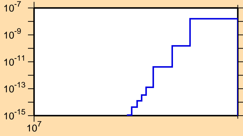
\sigma vs. E for ^{152}\text{Pr}(n,2n\alpha)
