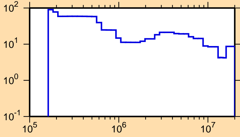
\Delta\sigma/\sigma vs. E for ^{152}\text{Pr}(n, el.)
