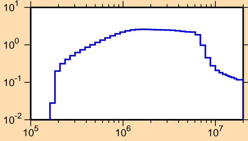
\sigma vs. E for ^{153}\text{Pr}(n,\text{inel.})
