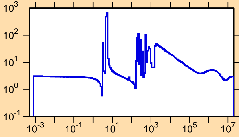
\sigma vs. E for ^{153}\text{Pr}(n,\text{el.})
