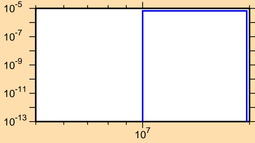
\sigma vs. E for ^{153}\text{Pr}(n,t)
