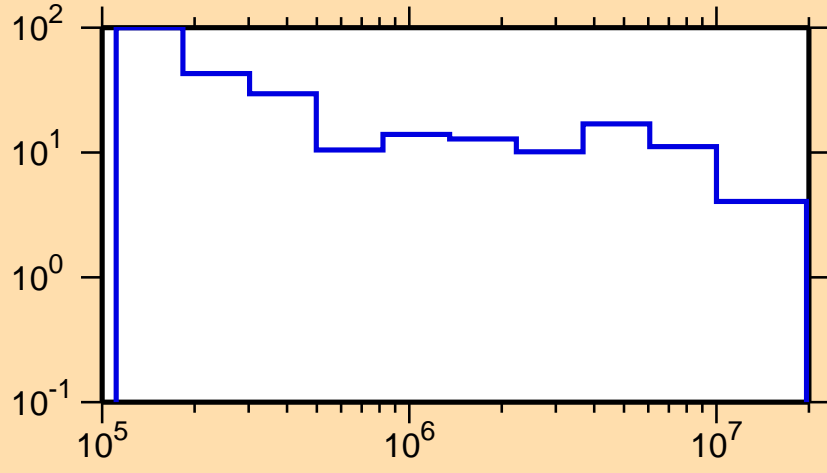
\Delta\sigma/\sigma vs. E for ^{153}\text{Pr}(n, tot.)
