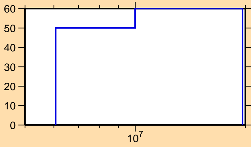
\Delta\sigma/\sigma vs. E for ^{153}\text{Pr}(n,ncont.)
