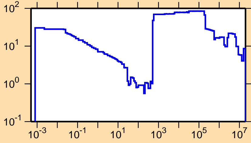
\Delta\sigma/\sigma vs. E for ^{154}\text{Pr}(n,\text{tot.})
