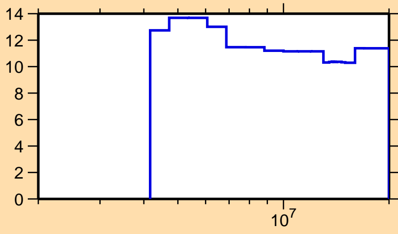
\Delta\sigma/\sigma vs. E for ^{154}\text{Pr}(n,\text{nonel.})
