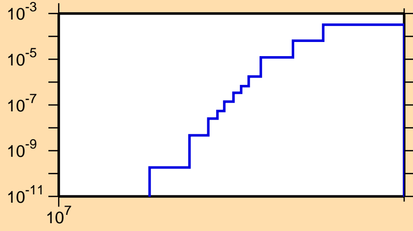
\sigma vs. E for ^{154}\text{Pr}(n,np)
