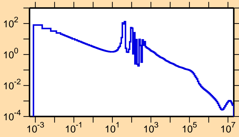
\sigma vs. E for ^{154}\text{Pr}(n,\gamma)
