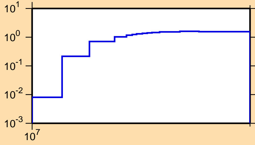
\sigma vs. E for ^{154}\text{Pr}(n,3n)
