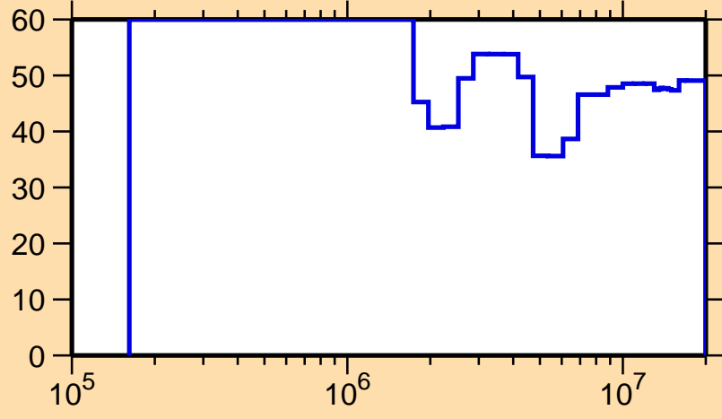
\Delta\sigma/\sigma vs. E for ^{154}\text{Pr}(n,n_1)
