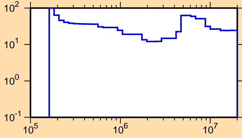
\Delta\sigma/\sigma vs. E for ^{154}\text{Pr}(n,\text{inel.})
