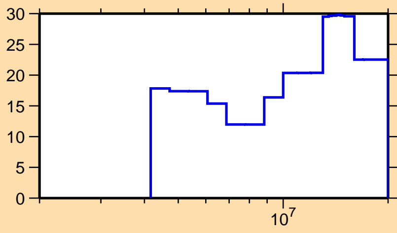
\Delta\sigma/\sigma vs. E for ^{154}\text{Pr}(n,2n)
