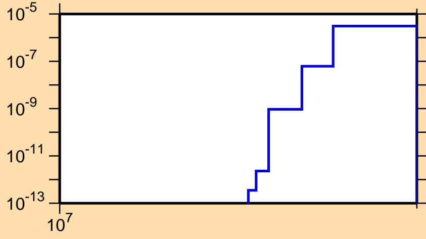
\sigma vs. E for ^{154}\text{Pr}(n,\text{nd})
