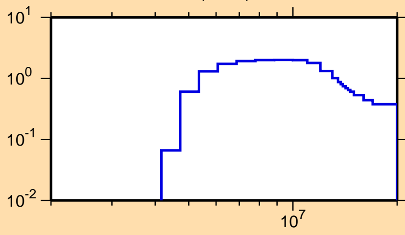
\sigma vs. E for ^{154}\text{Pr}(n,2n)
