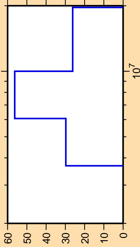
\Delta\sigma/\sigma vs. E for ^{154}\text{Pr}(n,n\text{cont.})
