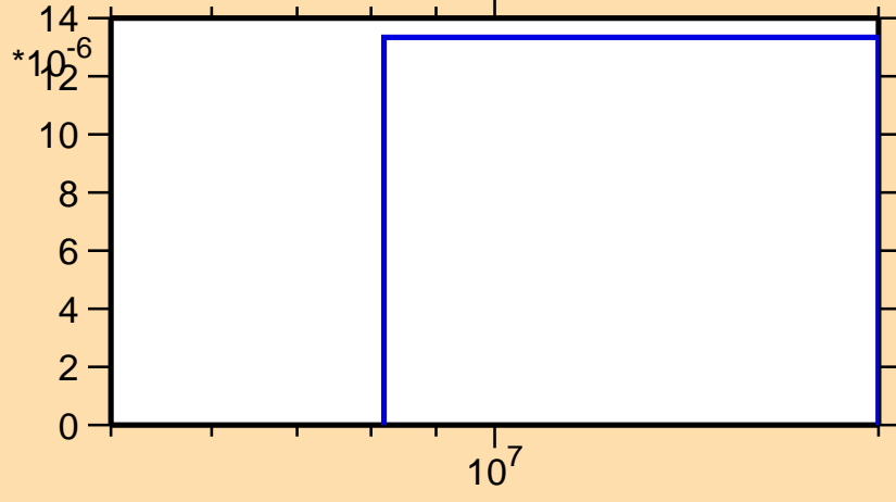
\sigma vs. E for ^{154}\text{Pr}(n,t)
