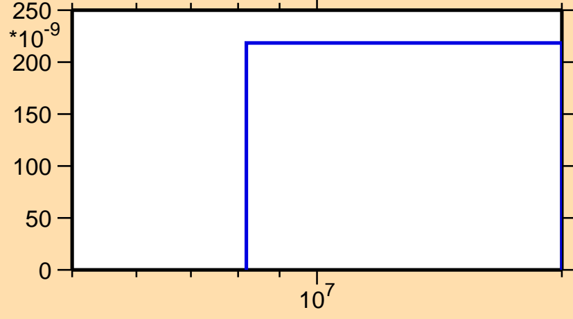
\sigma vs. E for ^{154}\text{Pr}(n,n\alpha)
