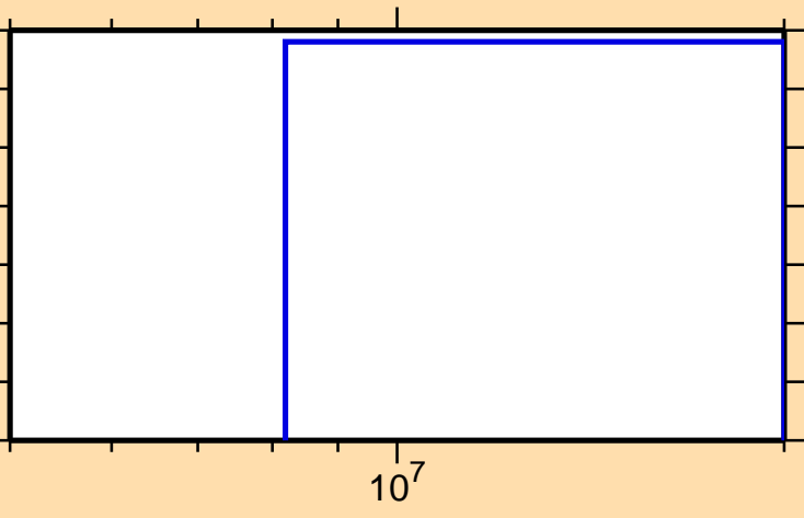
\sigma vs. E for ^{154}\text{Pr}(n,np)
