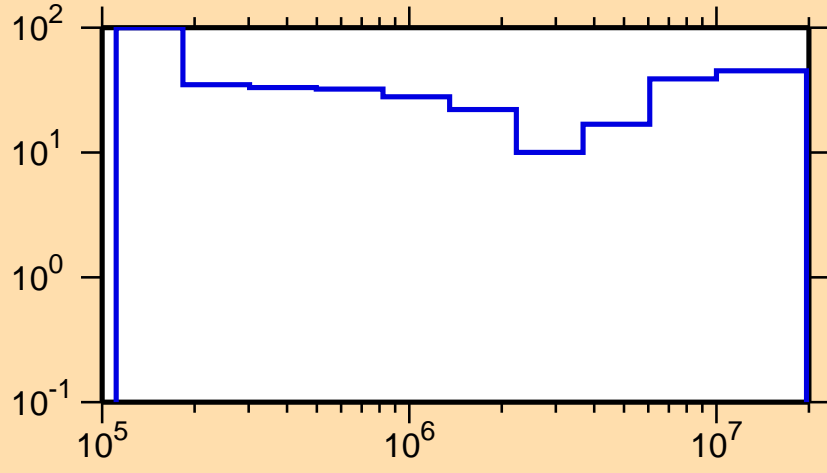
\Delta\sigma/\sigma vs. E for ^{155}\text{Pr}(n,\text{inel.})
