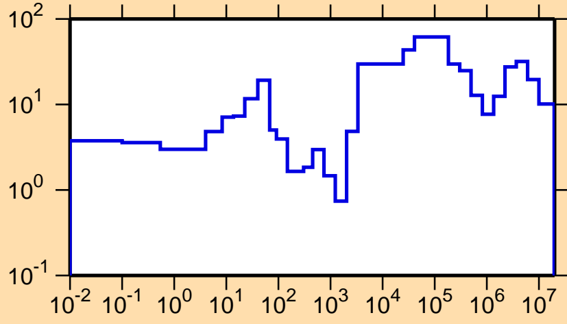
\Delta\sigma/\sigma vs. E for ^{155}\text{Pr}(n,\text{el.})
