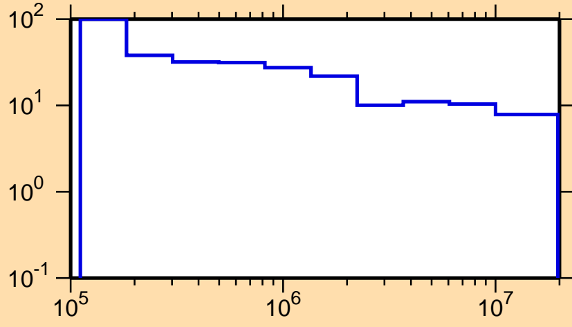
\Delta\sigma/\sigma vs. E for ^{155}\text{Pr}(n,\text{nonel.})
