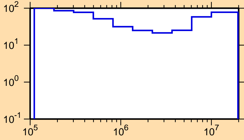
\Delta\sigma/\sigma vs. E for ^{155}\text{Pr}(n,n\text{cont.})
