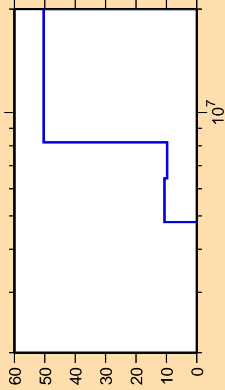
\Delta\sigma/\sigma vs. E for ^{155}\text{Pr}(n,2n)
