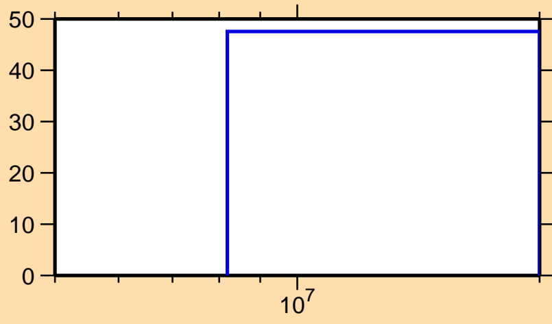
\Delta\sigma/\sigma vs. E for ^{155}\text{Pr}(n,\text{inel.})
