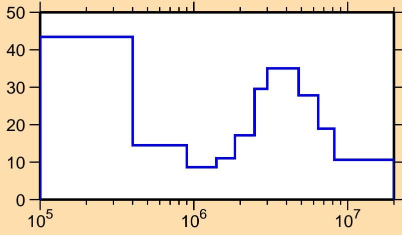
\Delta\sigma/\sigma vs. E for ^{155}\text{Pr}(n, el.)
