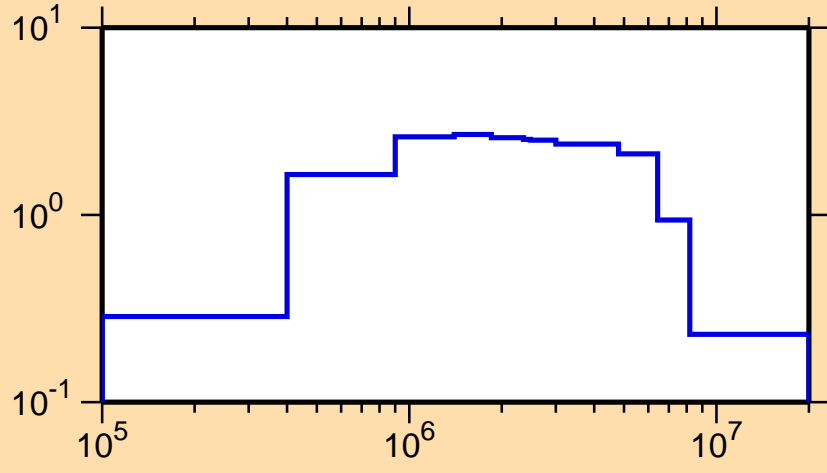
\sigma vs. E for ^{155}\text{Pr}(n,\text{inel.})
