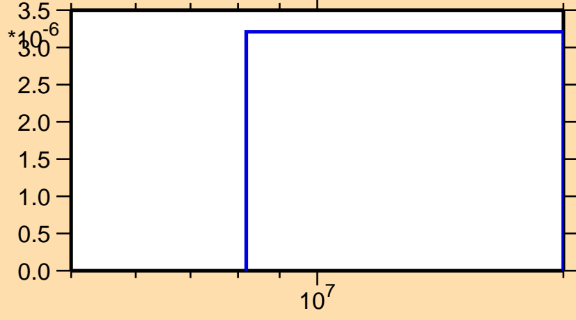
\sigma vs. E for ^{155}\text{Pr}(n,np)
