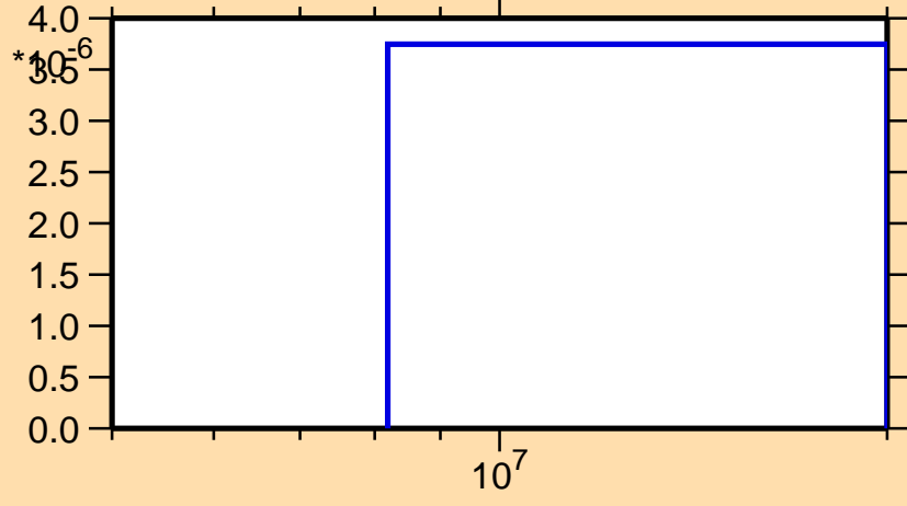
\sigma vs. E for ^{155}\text{Pr}(n,t)
