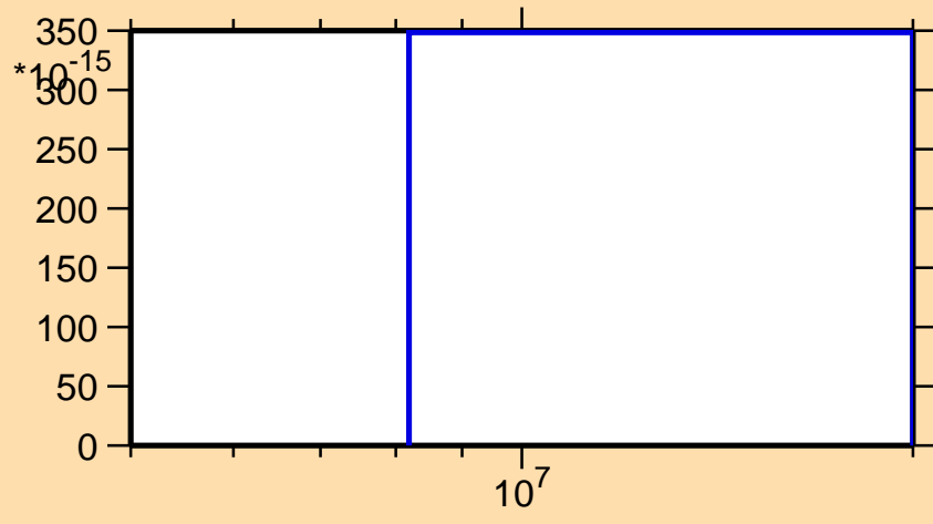
\sigma vs. E for ^{155}\text{Pr}(n,2n\alpha)
