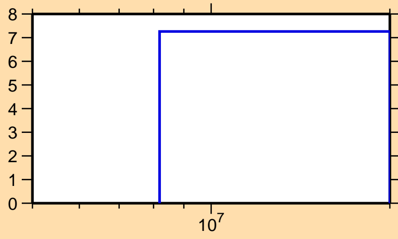
\Delta\sigma/\sigma vs. E for ^{155}\text{Pr}(n,\text{tot.})
