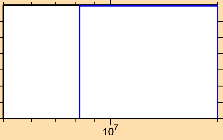
\sigma vs. E for ^{155}\text{Pr}(n,\alpha)
