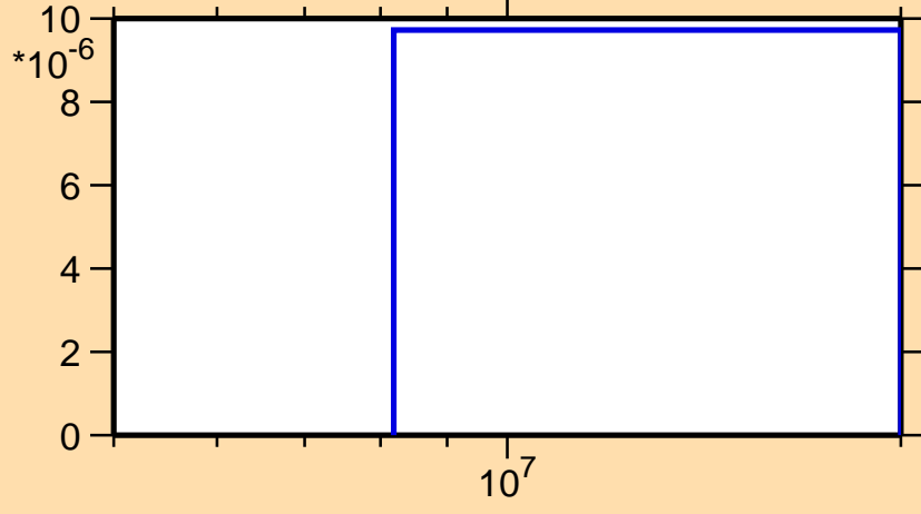
\sigma vs. E for ^{155}\text{Pr}(n,d)
