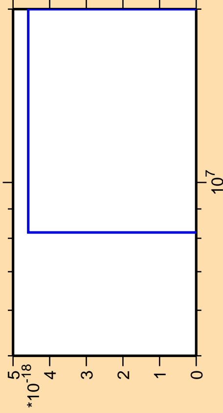
\Delta\sigma/\sigma vs. E for ^{155}\text{Pr}(\text{mt } 42)
