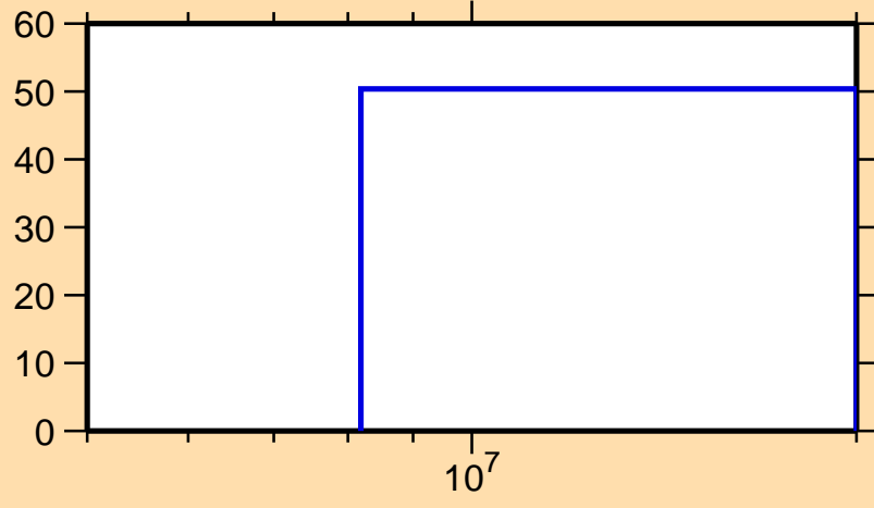
\Delta\sigma/\sigma vs. E for ^{155}\text{Pr}(n,2n)
