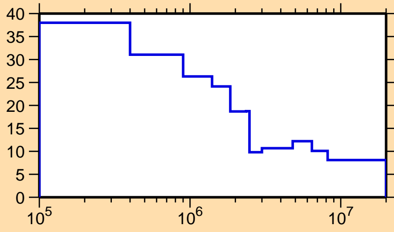
\Delta\sigma/\sigma vs. E for ^{155}\text{Pr}(n,\text{nonel.})
