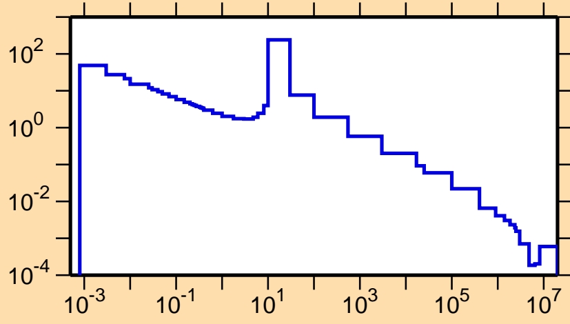
\sigma vs. E for ^{155}\text{Pr}(n,\gamma)
