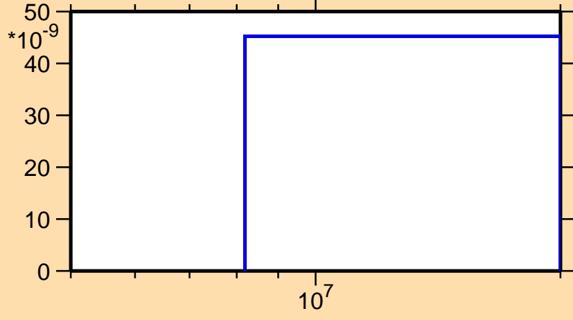
\sigma vs. E for ^{155}\text{Pr}(n,nt)
