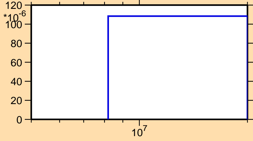
\sigma vs. E for ^{155}\text{Pr}(n,p)
