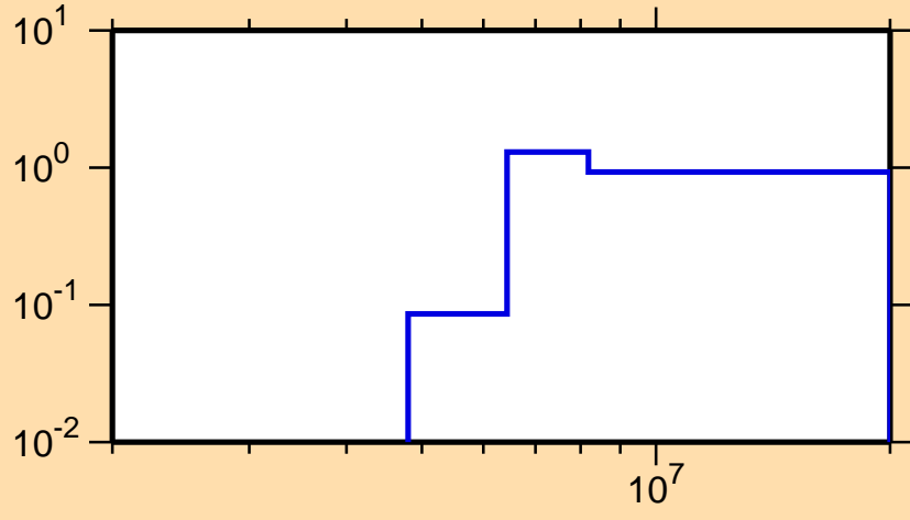
\sigma vs. E for ^{155}\text{Pr}(n,2n)
