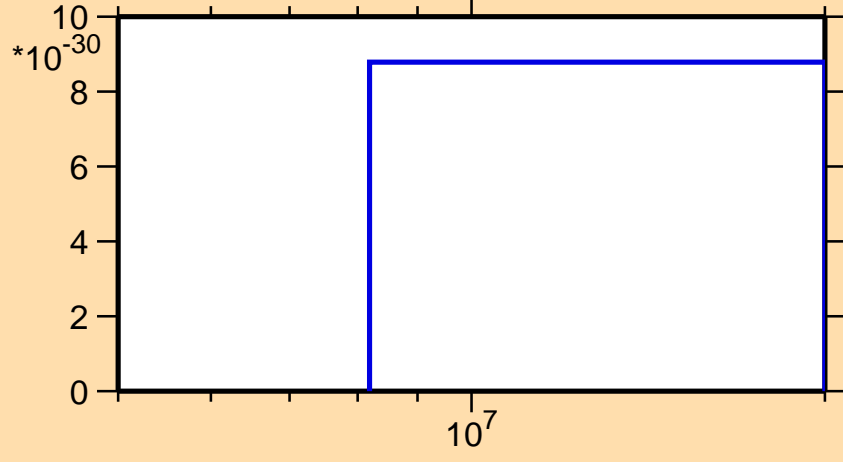
\sigma vs. E for ^{155}\text{Pr}(\text{mt } 42)
