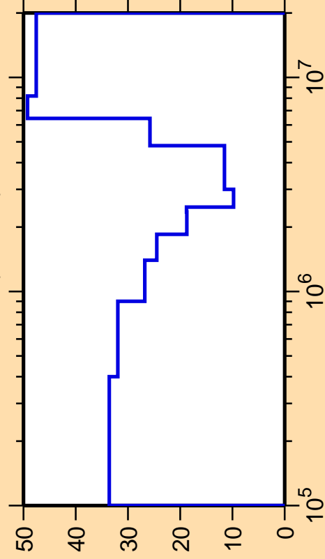
\Delta\sigma/\sigma vs. E for ^{155}\text{Pr}(n,\text{inel.})
