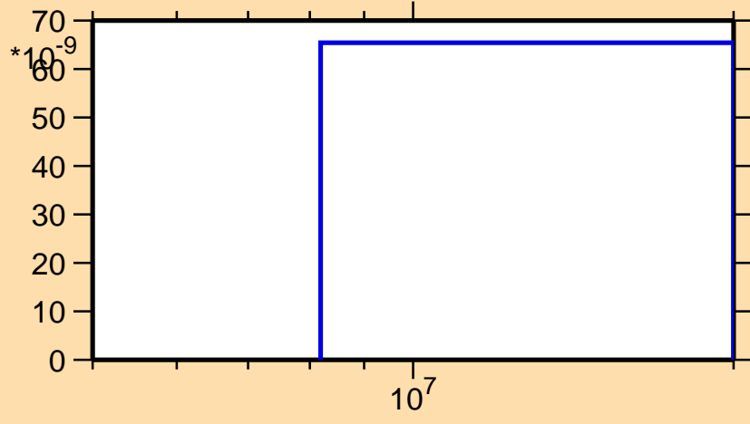
\sigma vs. E for ^{155}\text{Pr}(n,n\alpha)
