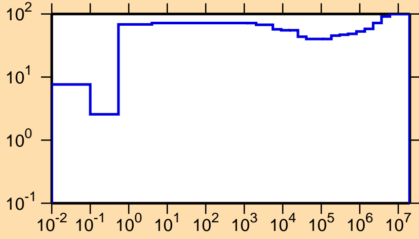
\Delta\sigma/\sigma vs. E for ^{175}\text{Pt}(n,\gamma)
