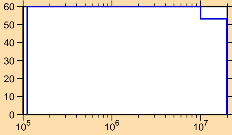
\Delta\sigma/\sigma vs. E for ^{175}\text{Pt}(n,ncont.)
