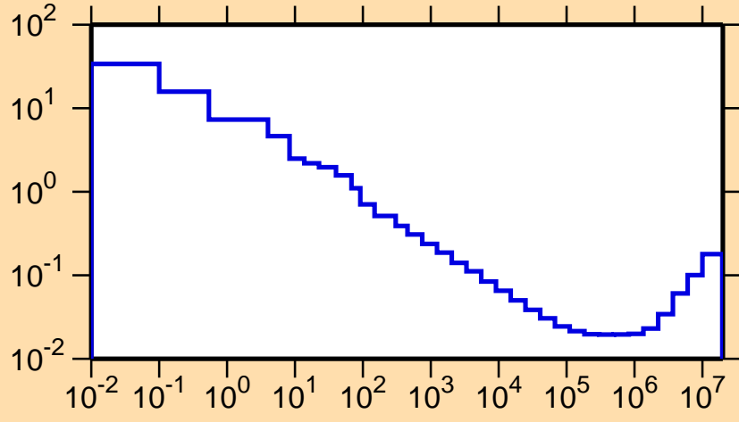
\sigma vs. E for ^{175}\text{Pt}(n,\alpha)
