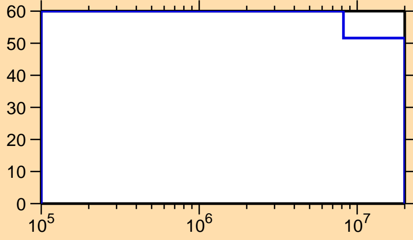
\Delta\sigma/\sigma vs. E for ^{175}\text{Pt}(n,n\text{cont.})
