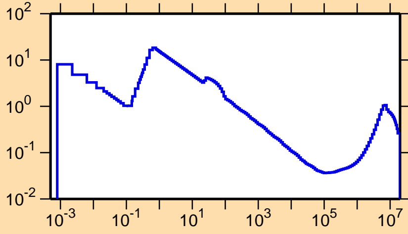
\sigma vs. E for ^{176}\text{Pt}(n,p)
