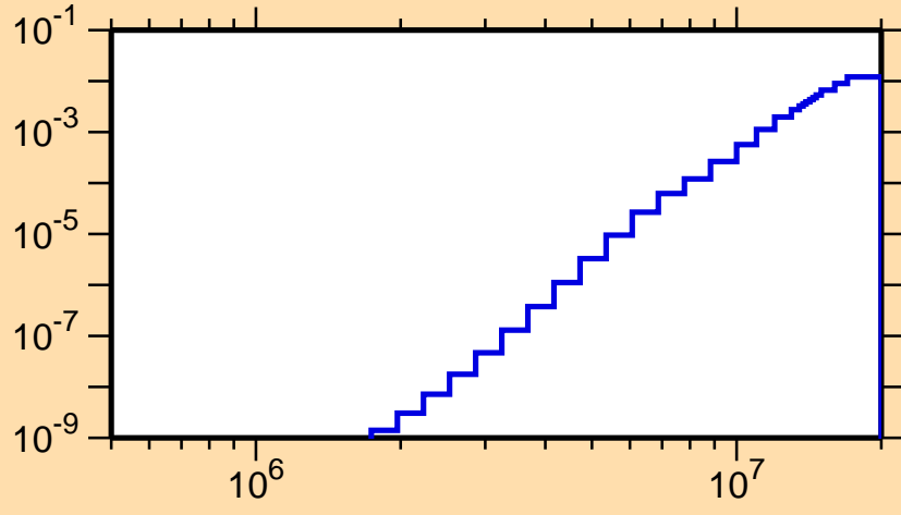
\sigma vs. E for ^{176}\text{Pt}(n, p\alpha)
