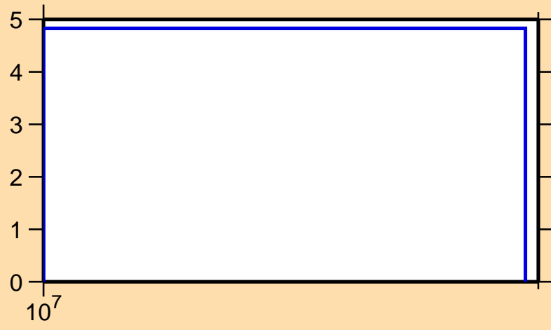
\Delta\sigma/\sigma vs. E for ^{176}\text{Pt}(n,\text{tot.})
