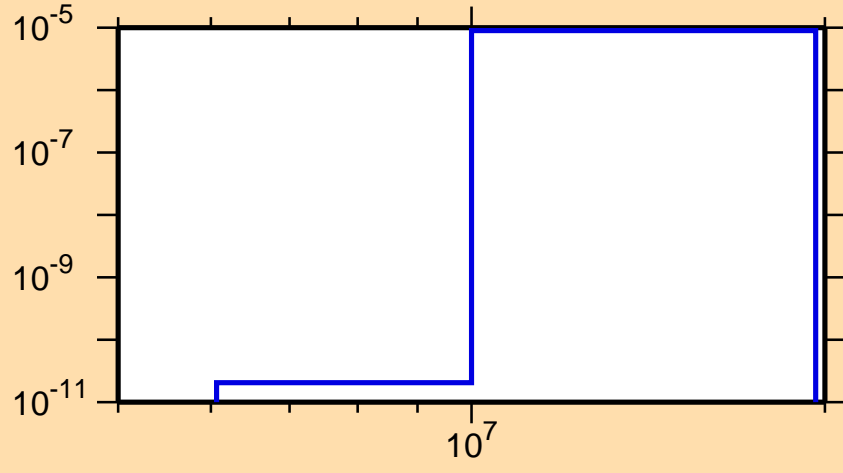
\sigma vs. E for ^{176}\text{Pt}(\text{mt } 45)
