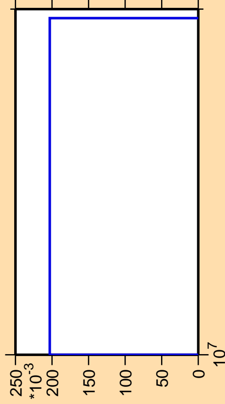
\Delta\sigma/\sigma vs. E for ^{176}\text{Pt}(n,nt)
