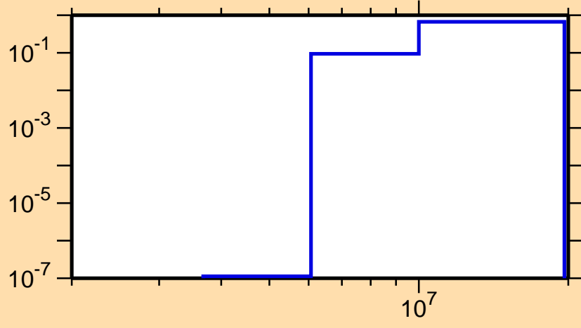
\sigma vs. E for ^{176}\text{Pt}(n,np)
