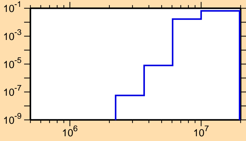
\sigma vs. E for ^{176}\text{Pt}(n,n\alpha)
