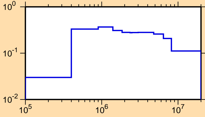
\sigma vs. E for ^{176}\text{Pt}(n,n_1)
