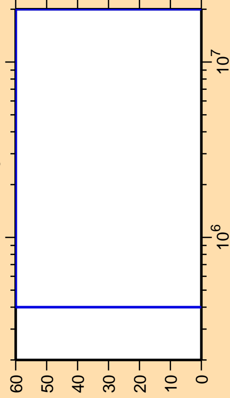
\Delta\sigma/\sigma vs. E for ^{176}\text{Pt}(n,n_3)
