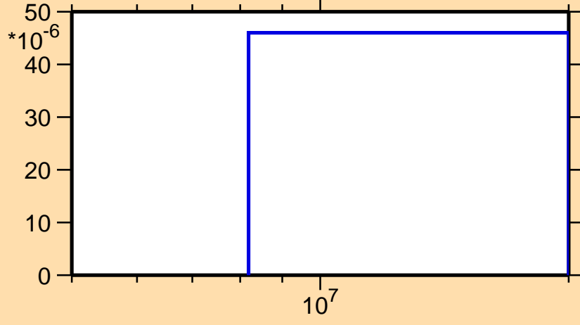
\sigma vs. E for ^{176}\text{Pt}(n,t)
