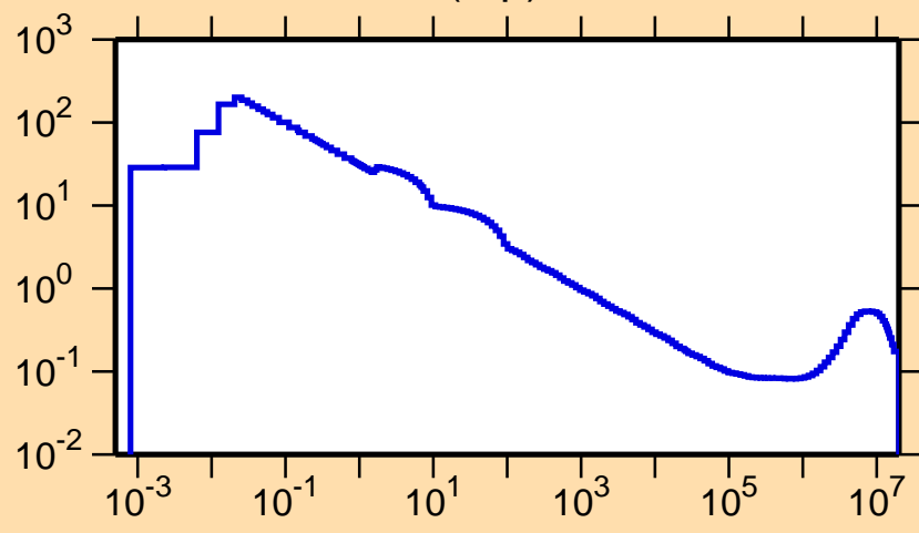
\sigma vs. E for ^{177}\text{Pt}(n,p)
