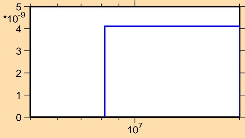
\sigma vs. E for ^{177}\text{Pt}(\text{mt117})
