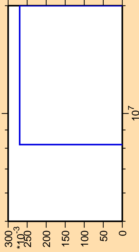
\Delta\sigma/\sigma vs. E for ^{177}\text{Pt}(n,3n)
