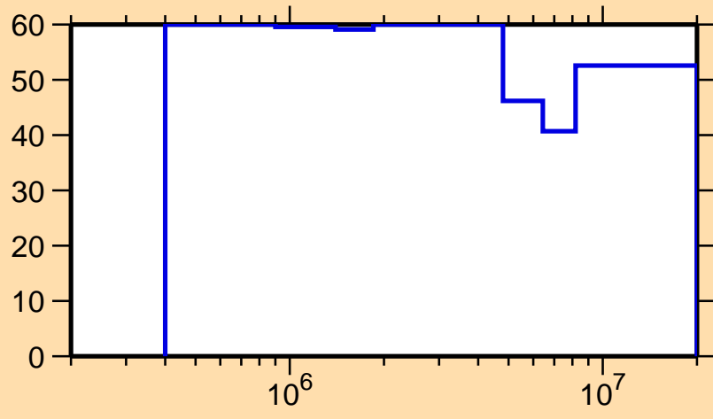
\Delta\sigma/\sigma vs. E for ^{177}\text{Pt}(n,ncont.)
