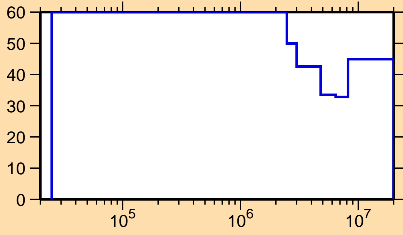
\Delta\sigma/\sigma vs. E for ^{177}\text{Pt}(n,\text{inel.})
