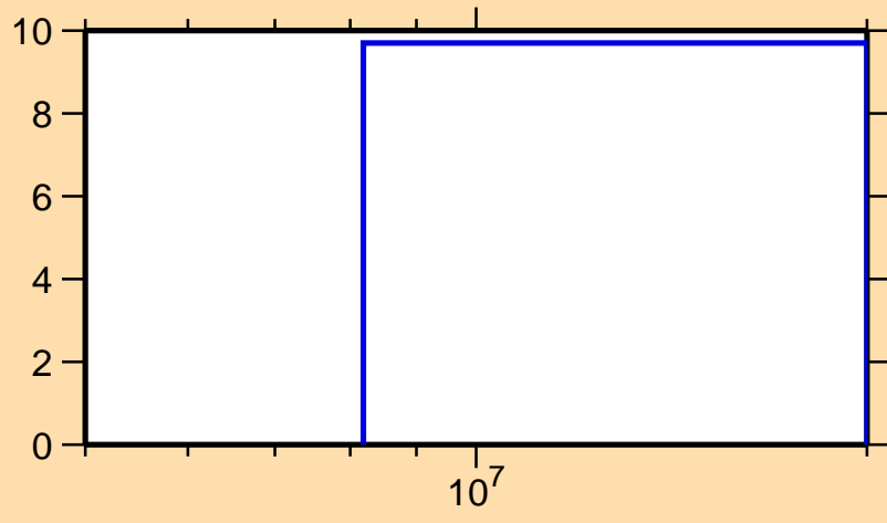
\Delta\sigma/\sigma vs. E for ^{177}\text{Pt}(n,\text{nonel.})
