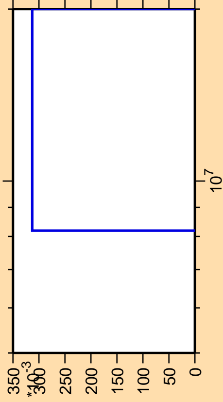
\Delta\sigma/\sigma vs. E for ^{177}\text{Pt}(n,nt)
