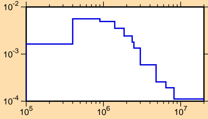
\sigma vs. E for ^{177}\text{Pt}(n,n_3)
