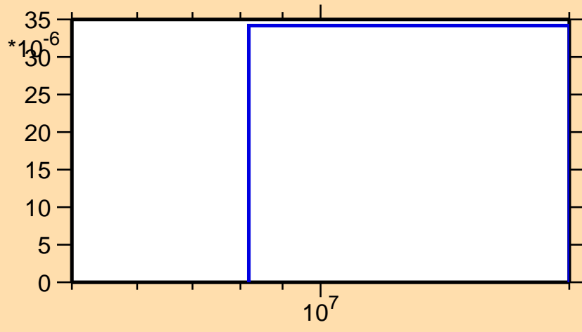
\sigma vs. E for ^{177}\text{Pt}(n,2np)
