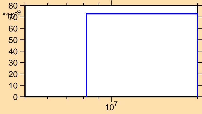
\sigma vs. E for ^{177}\text{Pt}(n,\text{nd})
