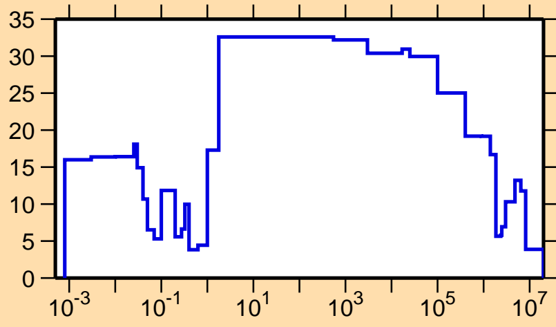
\Delta\sigma/\sigma vs. E for ^{177}\text{Pt}(n,\text{tot.})
