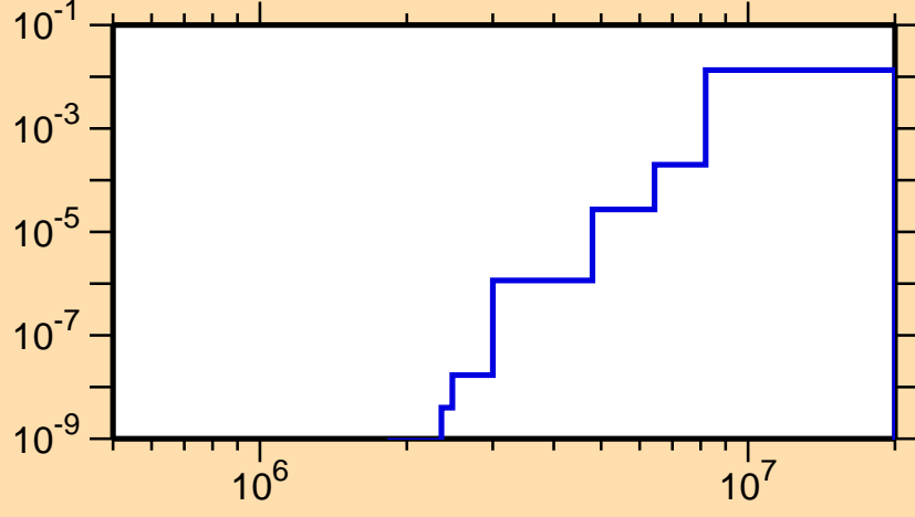
\sigma vs. E for ^{177}\text{Pt}(n,n\alpha)
