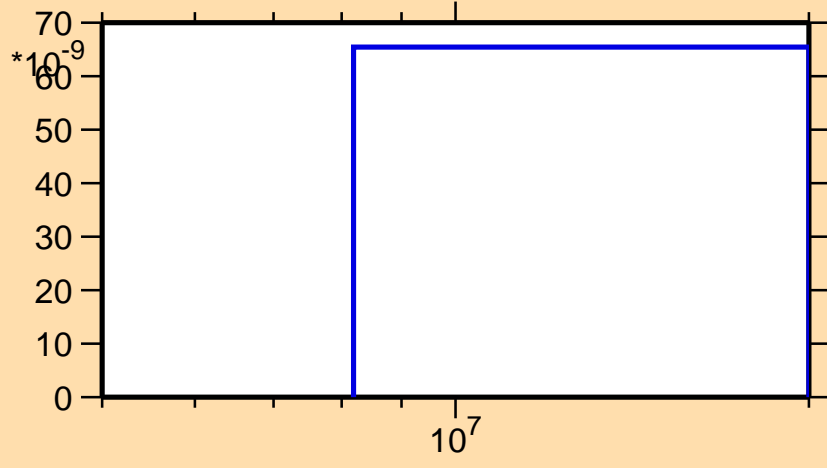
\sigma vs. E for ^{177}\text{Pt}(n,\text{pt})
