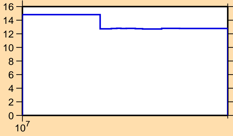
\Delta\sigma/\sigma vs. E for ^{178}\text{Pt}(n,\text{nonel.})
