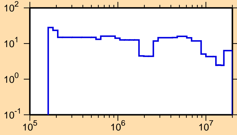
\Delta\sigma/\sigma vs. E for ^{178}\text{Pt}(n,\text{tot.})
