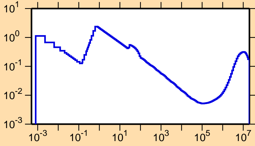
\sigma vs. E for ^{178}\text{Pt}(n,p)
