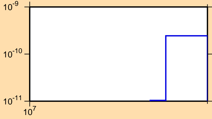
\sigma vs. E for ^{178}\text{Pt}(\text{mt } 34)
