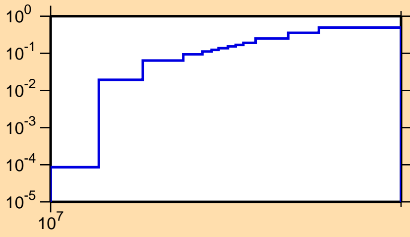
\sigma vs. E for ^{178}\text{Pt}(n,2n)
