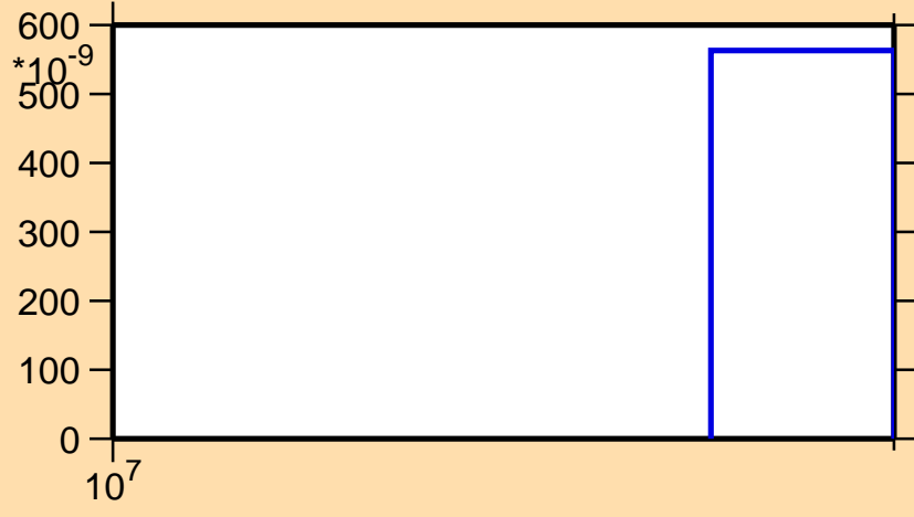
\sigma vs. E for ^{178}\text{Pt}(n,3n)
