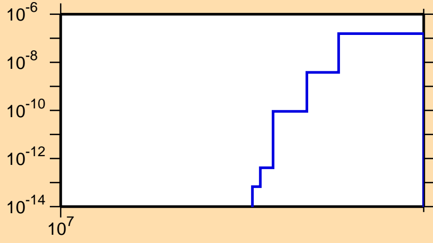
\sigma vs. E for ^{178}\text{Pt}(n,\text{nd})
