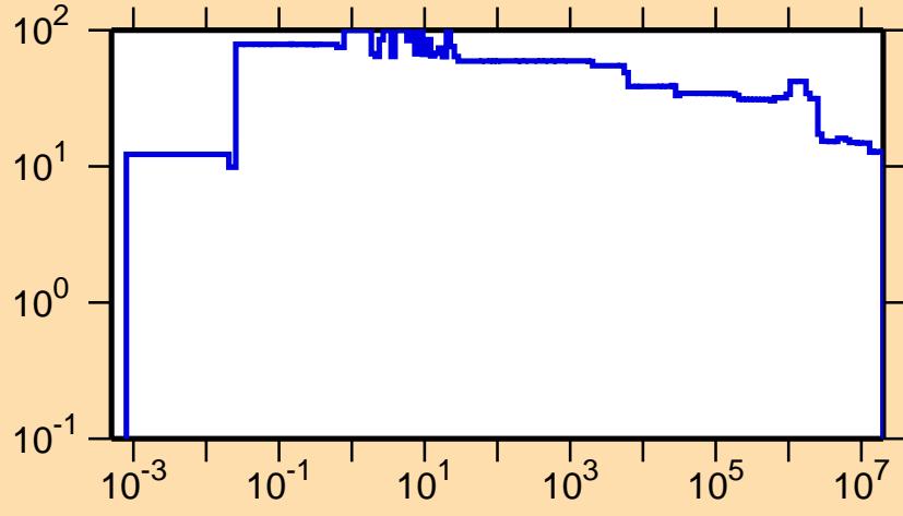
\Delta\sigma/\sigma vs. E for ^{178}\text{Pt}(n,\text{nonel.})
