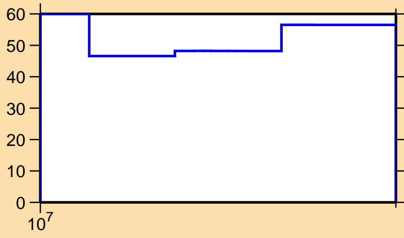
\Delta\sigma/\sigma vs. E for ^{178}\text{Pt}(n,2n)
