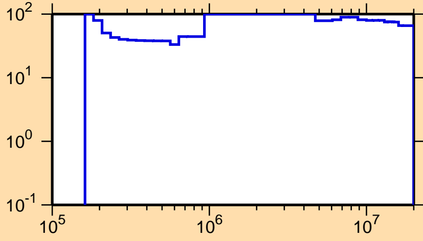
\Delta\sigma/\sigma vs. E for ^{178}\text{Pt}(n,n_1)
