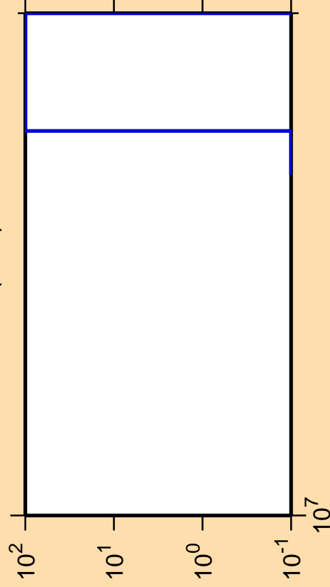
\Delta\sigma/\sigma vs. E for ^{178}\text{Pt}(n,nt)
