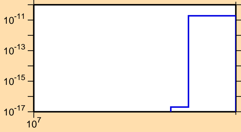
\sigma vs. E for ^{178}\text{Pt}(n,nt)
