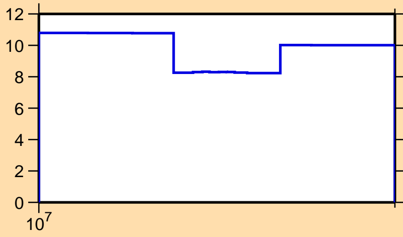
\Delta\sigma/\sigma vs. E for ^{178}\text{Pt}(n,\text{el.})
