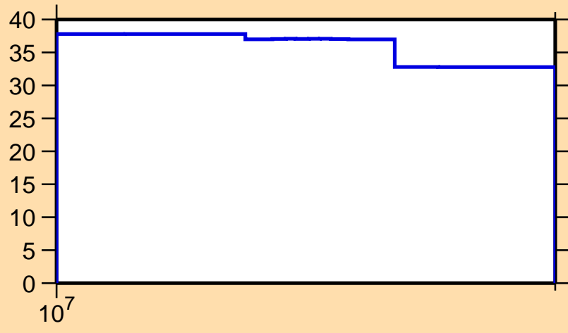
\Delta\sigma/\sigma vs. E for ^{178}\text{Pt}(n,\text{inel.})
