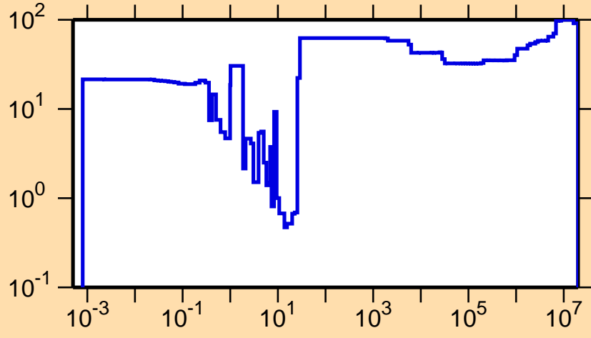
\Delta\sigma/\sigma vs. E for ^{178}\text{Pt}(n,\gamma)
