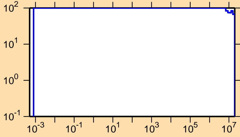
\Delta\sigma/\sigma vs. E for ^{178}\text{Pt}(n,p)
