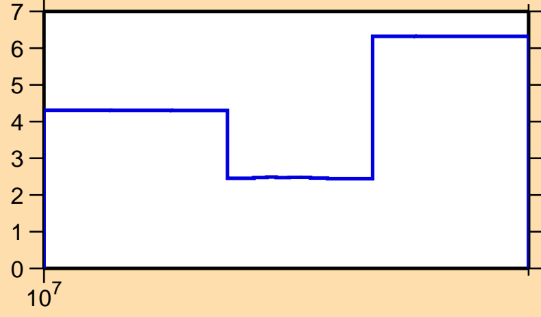
\Delta\sigma/\sigma vs. E for ^{178}\text{Pt}(n,\text{tot.})
