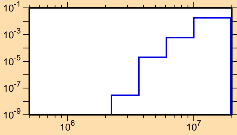
\sigma vs. E for ^{178}\text{Pt}(n,n\alpha)
