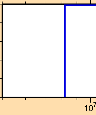
\sigma vs. E for ^{178}\text{Pt}(n,t)
