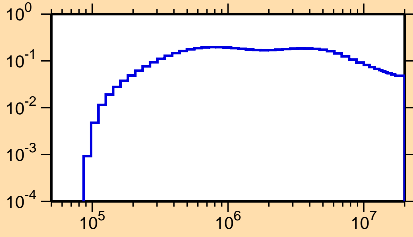
\sigma vs. E for ^{179}\text{Pt}(n,n_2)
