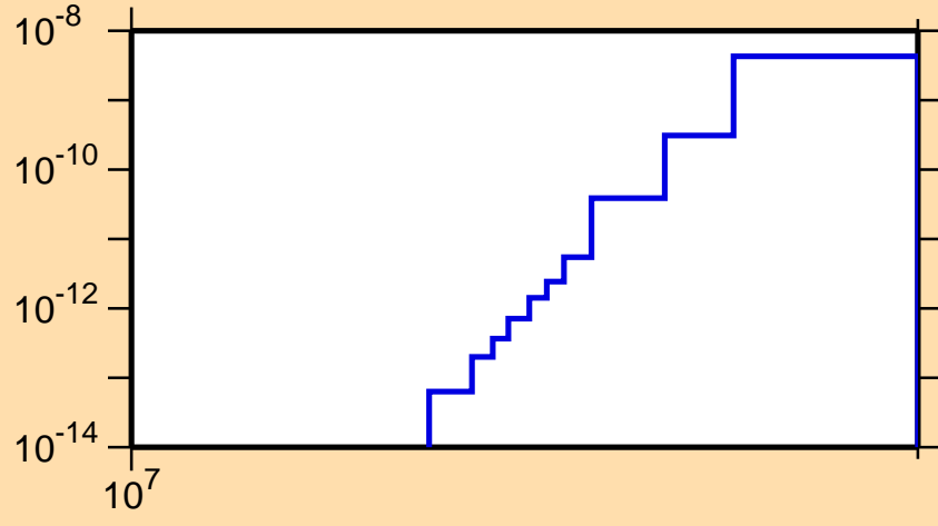
\sigma vs. E for ^{179}\text{Pt}(\text{mt } 34)
