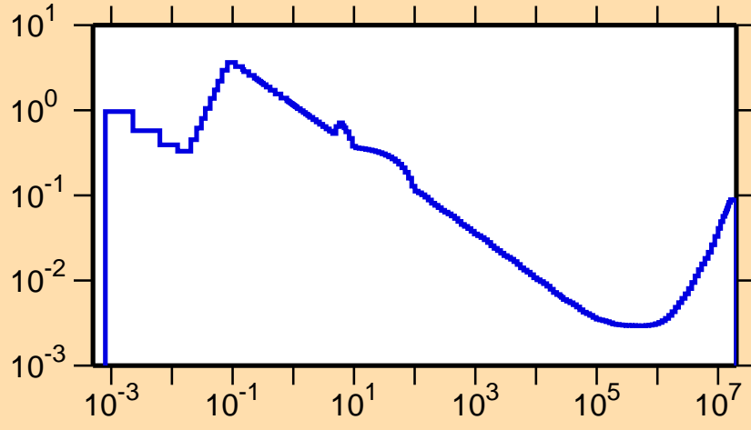
\sigma vs. E for ^{179}\text{Pt}(n,\alpha)
