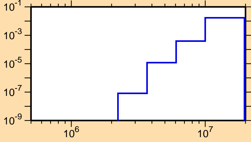
\sigma vs. E for ^{179}\text{Pt}(n,n\alpha)
