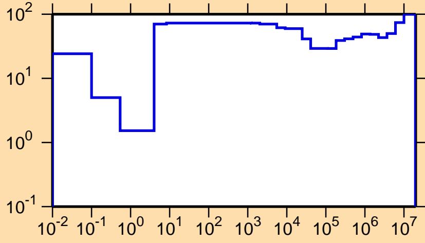
\Delta\sigma/\sigma vs. E for ^{179}\text{Pt}(n,\gamma)
