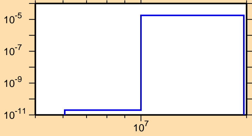
\sigma vs. E for ^{179}\text{Pt}(n,2n\alpha)
