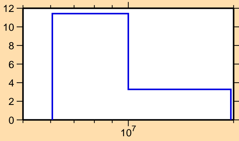
\Delta\sigma/\sigma vs. E for ^{179}\text{Pt}(n,\text{tot.})
