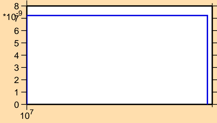
\sigma vs. E for ^{179}\text{Pt}(n,\text{pt})
