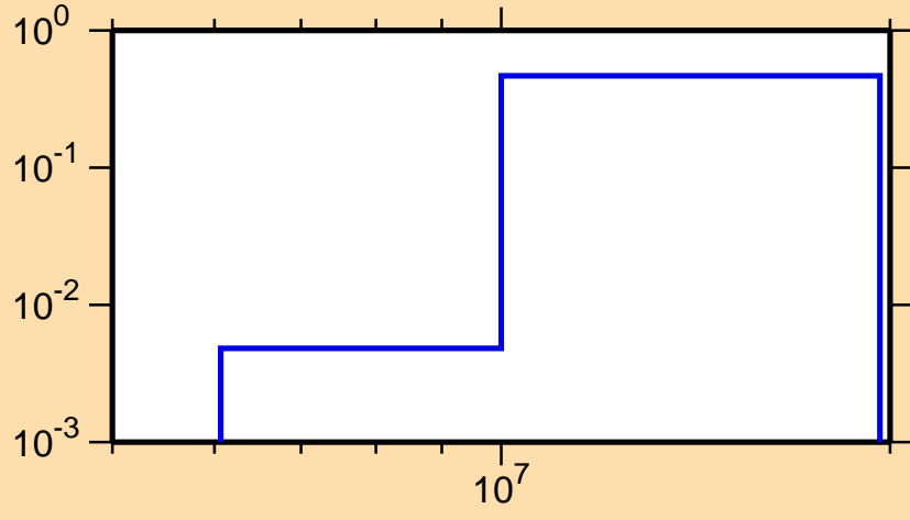
\sigma vs. E for ^{179}\text{Pt}(n,2n)
