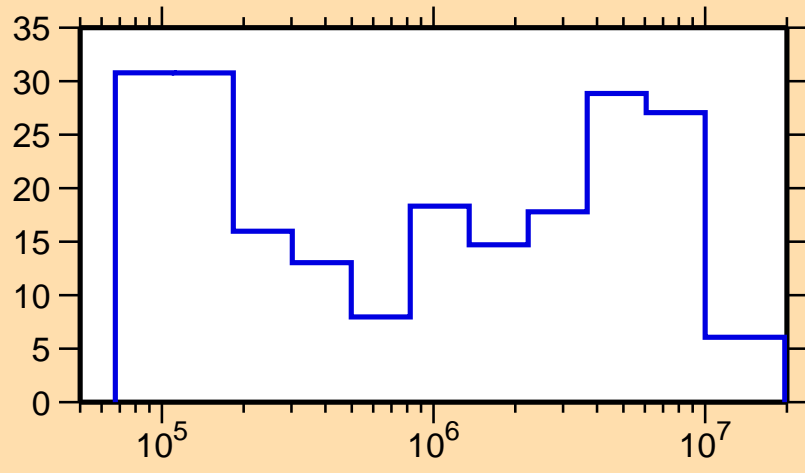
\Delta\sigma/\sigma vs. E for ^{179}\text{Pt}(n,\text{el.})
