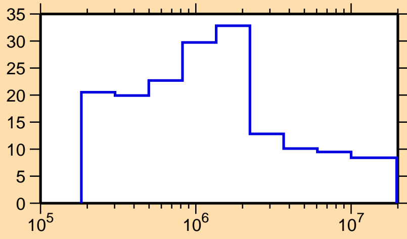
\Delta\sigma/\sigma vs. E for ^{179}\text{Pt}(n,\text{nonel.})
