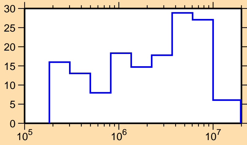
\Delta\sigma/\sigma vs. E for ^{179}\text{Pt}(n, el.)
