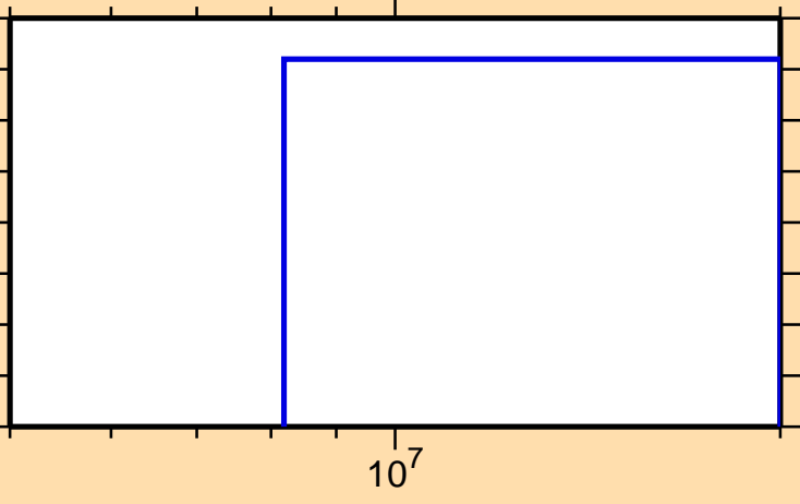
\sigma vs. E for ^{179}\text{Pt}(n,2n\alpha)
