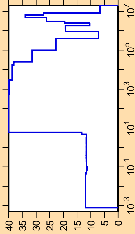
\Delta\sigma/\sigma vs. E for ^{179}\text{Pt}(n,\text{el.})
