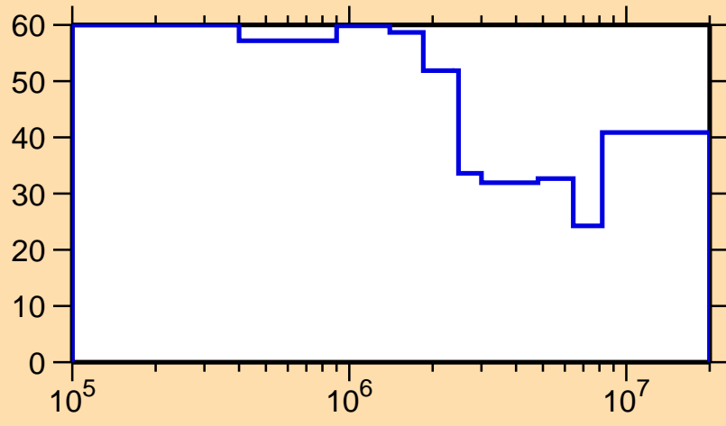
\Delta\sigma/\sigma vs. E for ^{179}\text{Pt}(n,n\text{cont.})
