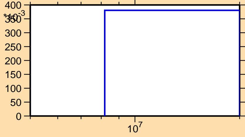
\sigma vs. E for ^{179}\text{Pt}(n,2n)
