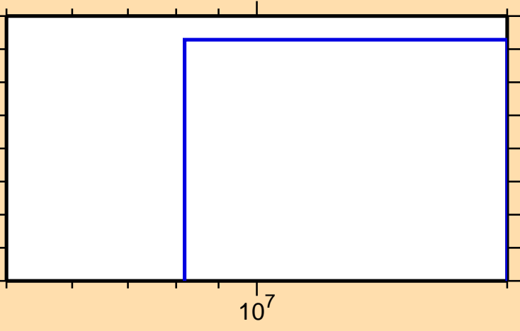
\sigma vs. E for ^{179}\text{Pt}(n,2np)
