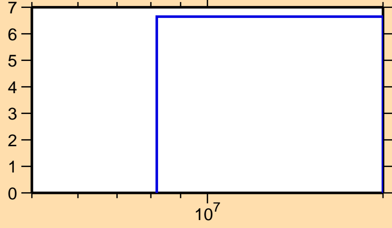
\Delta\sigma/\sigma vs. E for ^{179}\text{Pt}(n,\text{el.})
