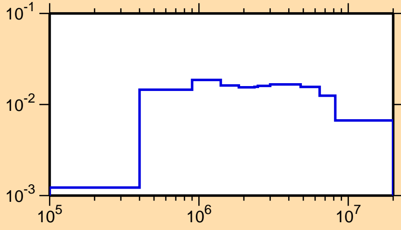
\sigma vs. E for ^{179}\text{Pt}(n,n_4)
