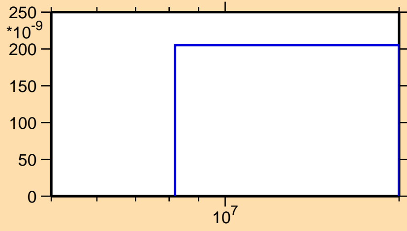
\sigma vs. E for ^{179}\text{Pt}(\text{mt } 45)
