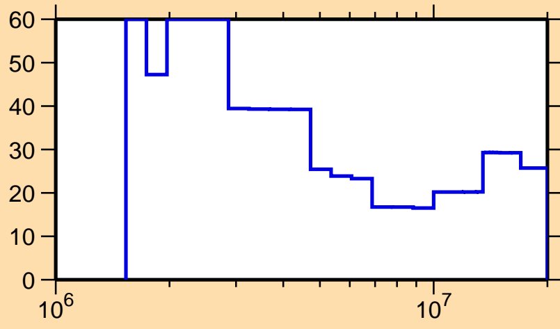
\Delta\sigma/\sigma vs. E for ^{180}\text{Pt}(n,n\text{cont.})
