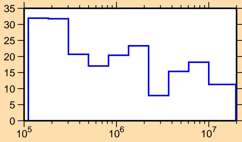
\Delta\sigma/\sigma vs. E for ^{180}\text{Pt}(n,\text{el.})
