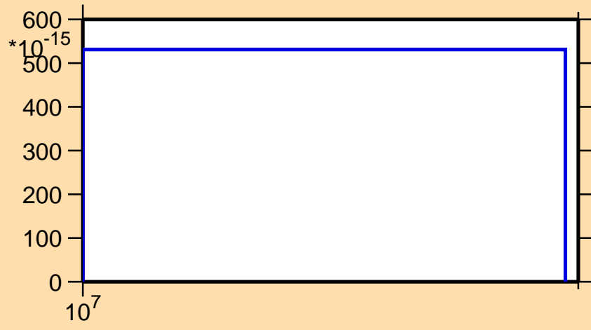
\sigma vs. E for ^{180}\text{Pt}(\text{mt } 34)
