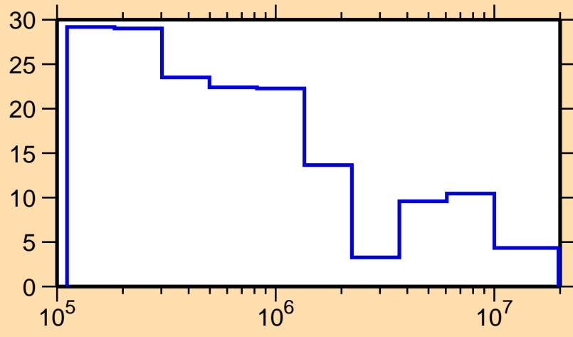
\Delta\sigma/\sigma vs. E for ^{180}\text{Pt}(n,\text{tot.})
