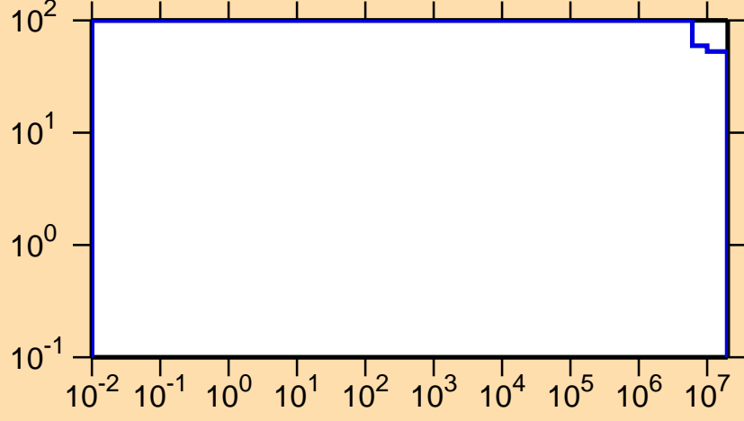
\Delta\sigma/\sigma vs. E for ^{180}\text{Pt}(n,p)
