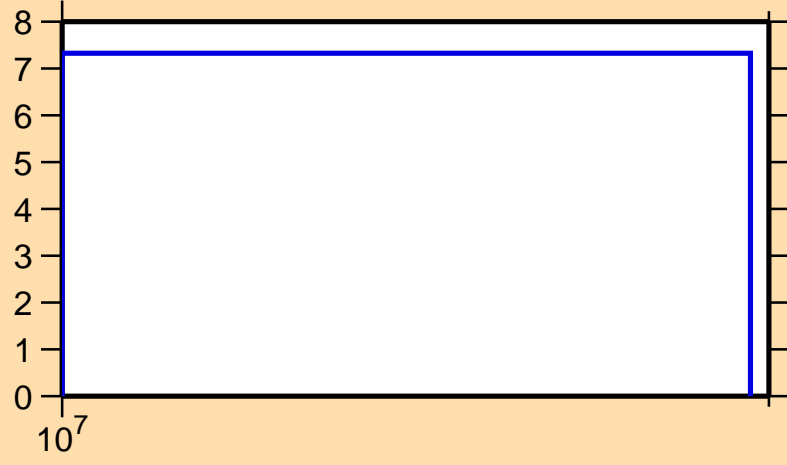
\Delta\sigma/\sigma vs. E for ^{180}\text{Pt}(n,\text{nonel.})
