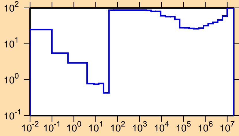
\Delta\sigma/\sigma vs. E for ^{180}\text{Pt}(n,\gamma)
