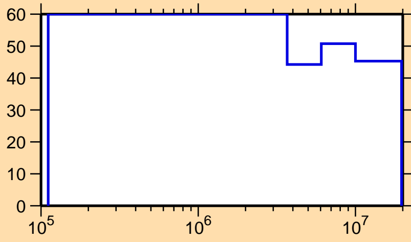
\Delta\sigma/\sigma vs. E for ^{180}\text{Pt}(n,n_1)
