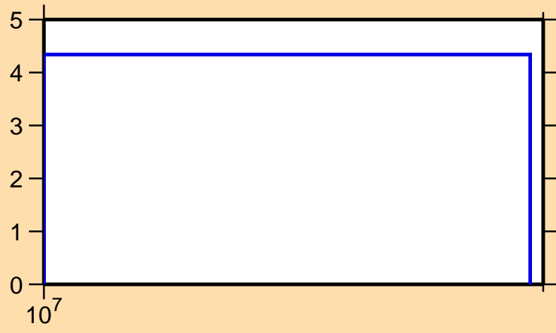
\Delta\sigma/\sigma vs. E for ^{180}\text{Pt}(n,\text{tot.})
