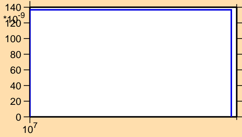
\sigma vs. E for ^{180}\text{Pt}(n,3n)
