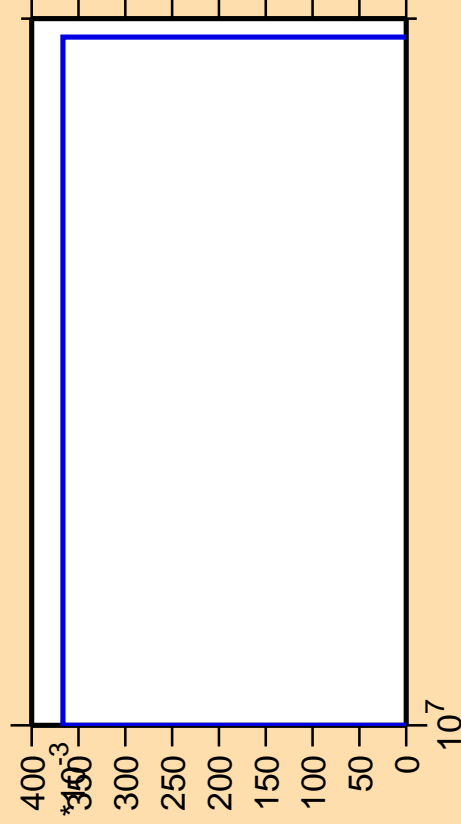
\Delta\sigma/\sigma vs. E for ^{180}\text{Pt}(n,nt)
