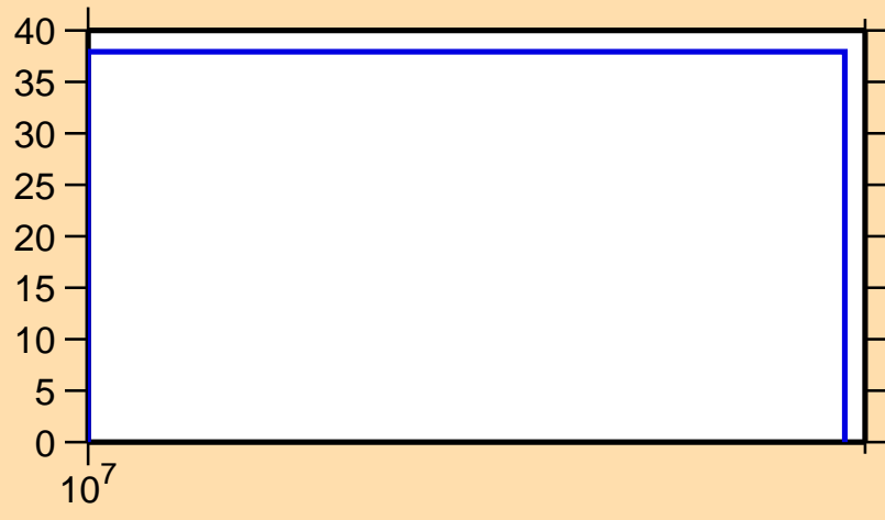
\Delta\sigma/\sigma vs. E for ^{180}\text{Pt}(n,2n)
