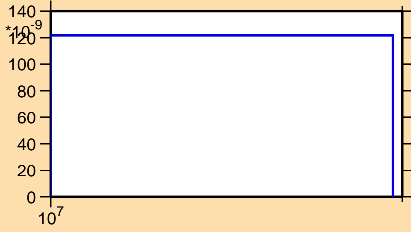
\sigma vs. E for ^{180}\text{Pt}(n,2np)
