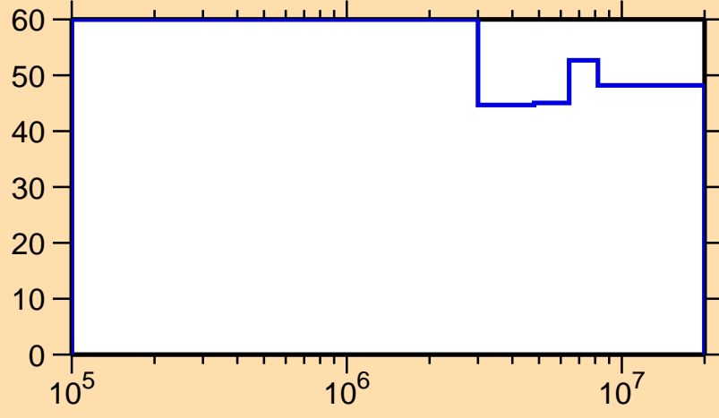
\Delta\sigma/\sigma vs. E for ^{180}\text{Pt}(n,n_1)
