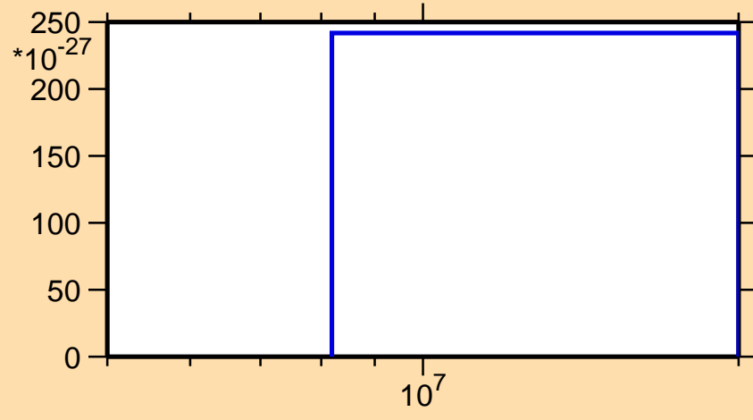
\sigma vs. E for ^{180}\text{Pt}(\text{mt } 11)
