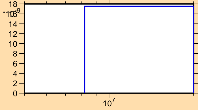
\sigma vs. E for ^{180}\text{Pt}(n,\text{pd})
