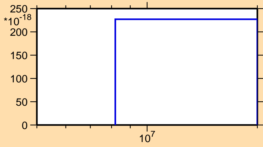
\sigma vs. E for ^{180}\text{Pt}(n,3n\alpha)
