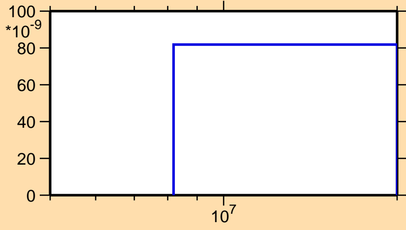
\sigma vs. E for ^{180}\text{Pt}(\text{mt } 45)
