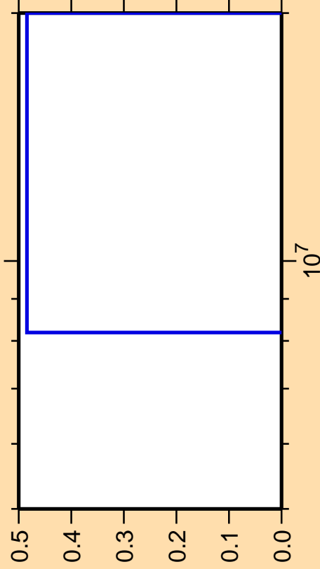
\Delta\sigma/\sigma vs. E for ^{180}\text{Pt}(n,nt)
