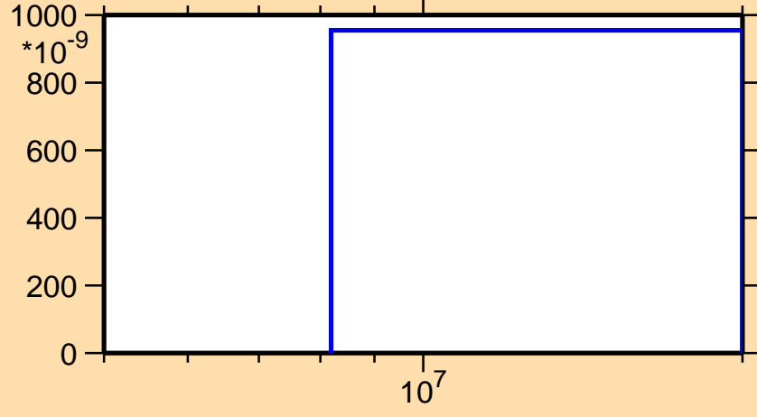
\sigma vs. E for ^{180}\text{Pt}(n,2n\alpha)
