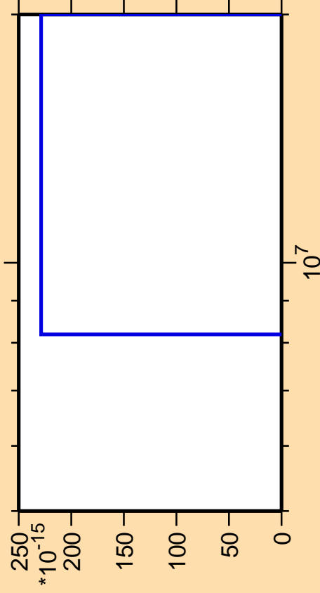
\Delta\sigma/\sigma vs. E for ^{180}\text{Pt}(\text{mt } 11)
