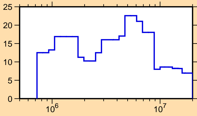
\Delta\sigma/\sigma vs. E for ^{181}\text{Pt}(n, el.)
