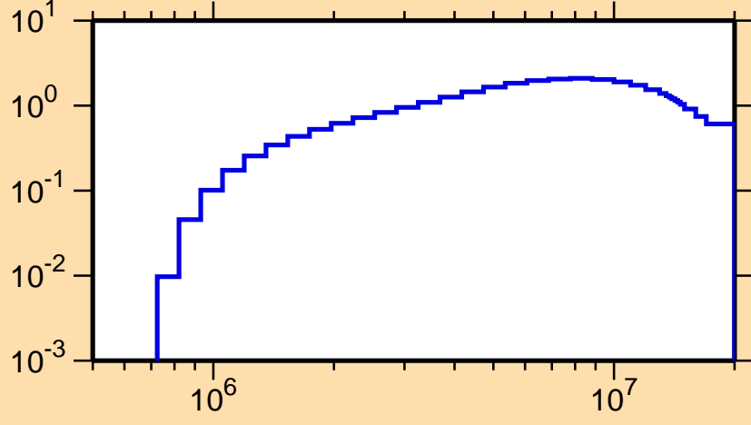
\sigma vs. E for ^{181}\text{Pt}(n,n\text{cont.})
