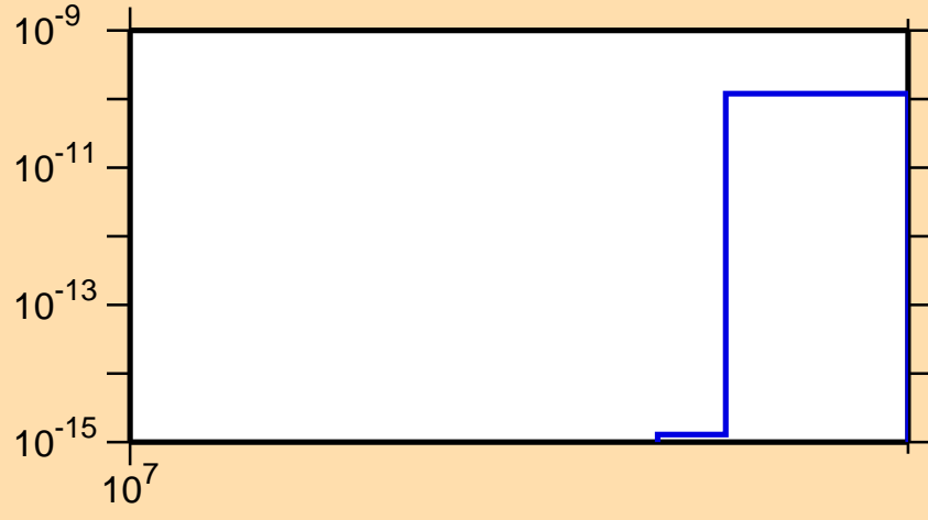
\sigma vs. E for ^{181}\text{Pt}(n,nt)
