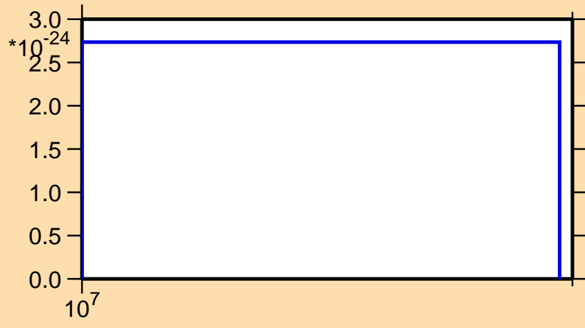
\sigma vs. E for ^{181}\text{Pt}(\text{mt } 11)
