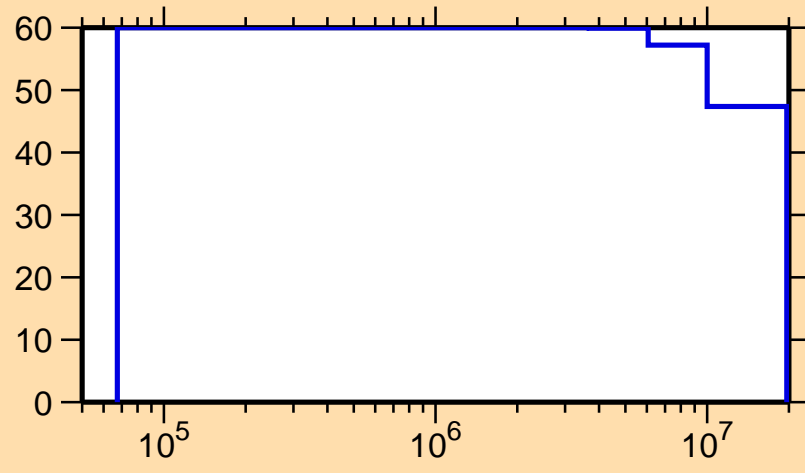
\Delta\sigma/\sigma vs. E for ^{181}\text{Pt}(n,n_1)
