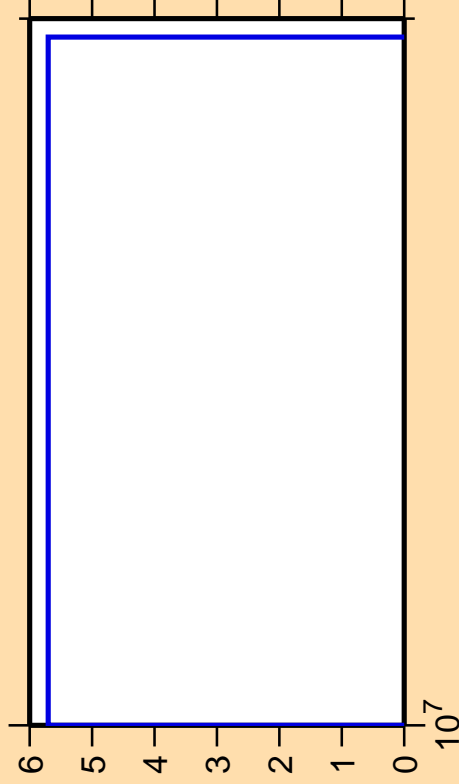
\Delta\sigma/\sigma vs. E for ^{181}\text{Pt}(n,nt)
