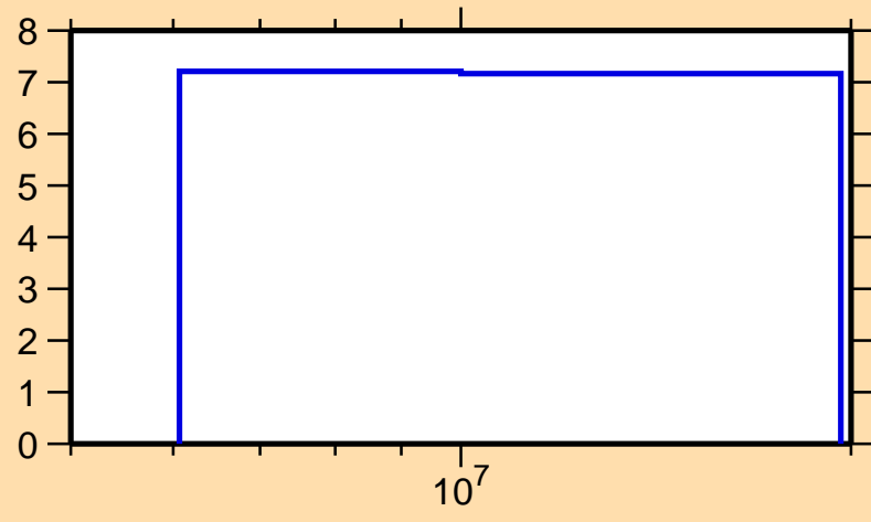
\Delta\sigma/\sigma vs. E for ^{181}\text{Pt}(n,\text{nonel.})
