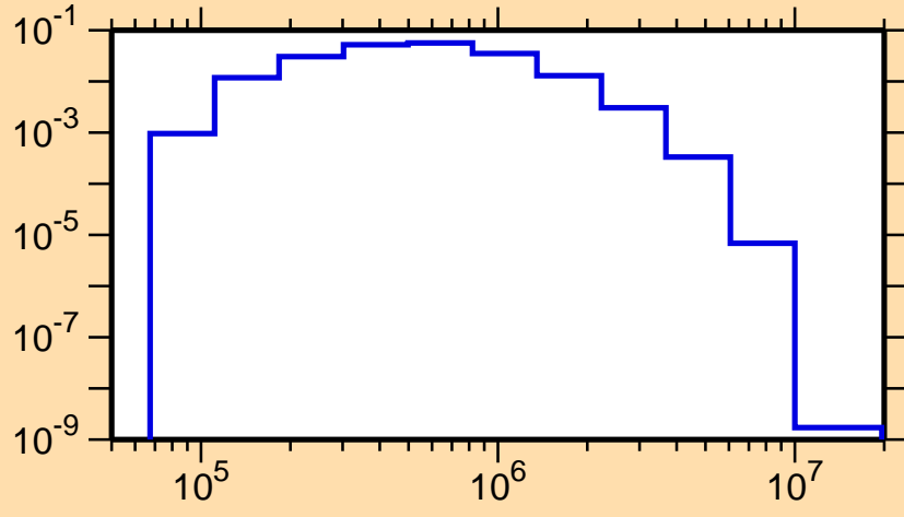
\sigma vs. E for ^{181}\text{Pt}(n,n_2)
