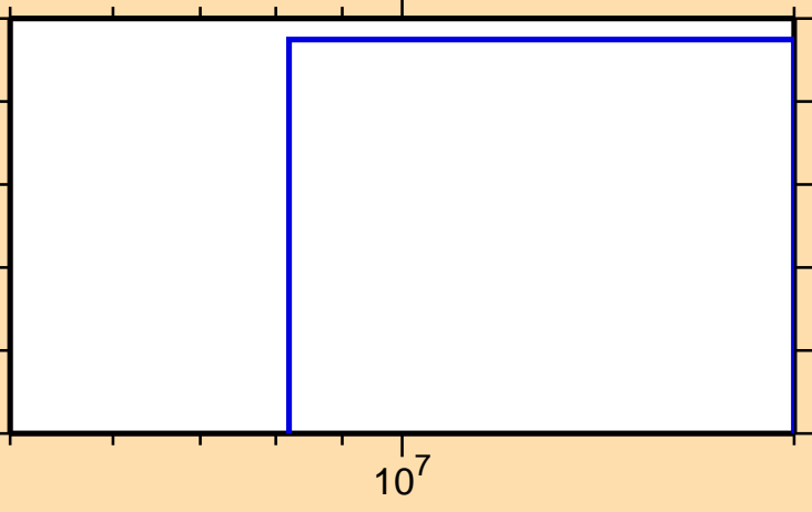
\sigma vs. E for ^{182}\text{Pt}(n,3n)
