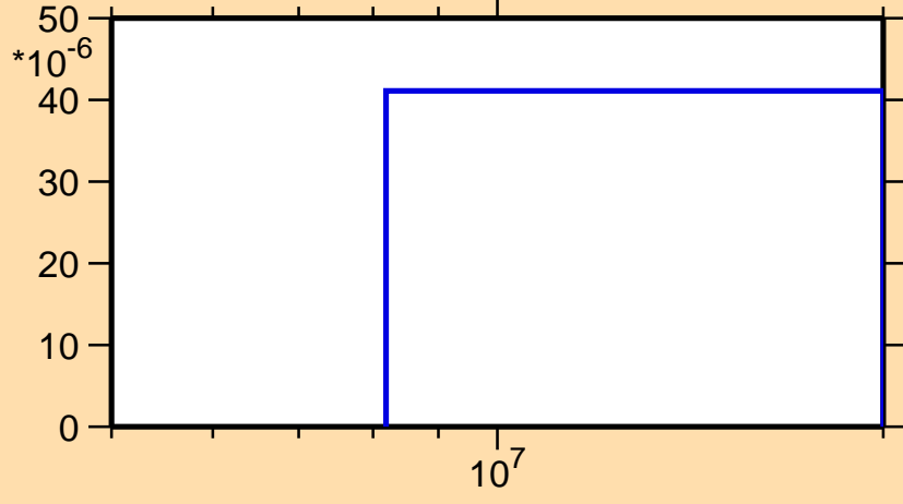
\sigma vs. E for ^{182}\text{Pt}(n,t)
