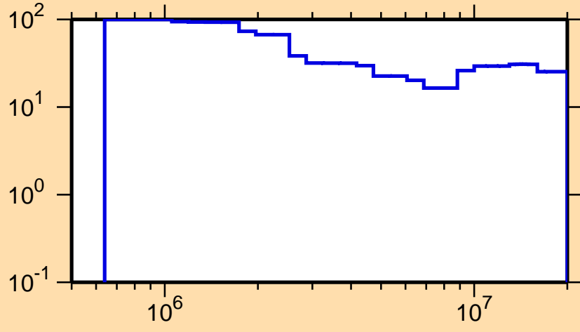
\Delta\sigma/\sigma vs. E for ^{183}\text{Pt}(n,n\text{cont.})
