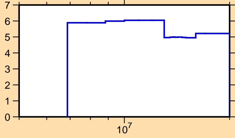
\Delta\sigma/\sigma vs. E for ^{183}\text{Pt}(n,\text{nonel.})
