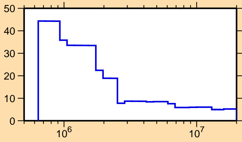
\Delta\sigma/\sigma vs. E for ^{183}\text{Pt}(n,\text{nonel.})
