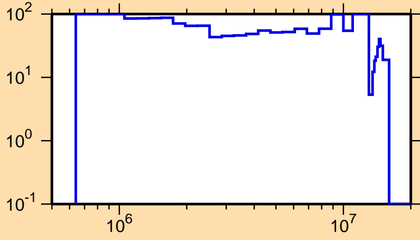
\Delta\sigma/\sigma vs. E for ^{183}\text{Pt}(n,n_1)
