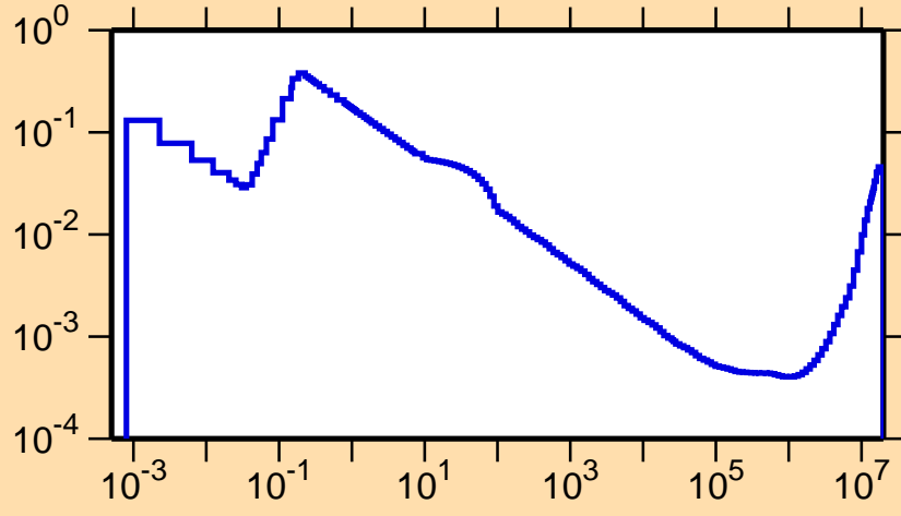
\sigma vs. E for ^{183}\text{Pt}(n,\alpha)
