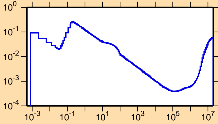
\sigma vs. E for ^{183}\text{Pt}(n,p)
