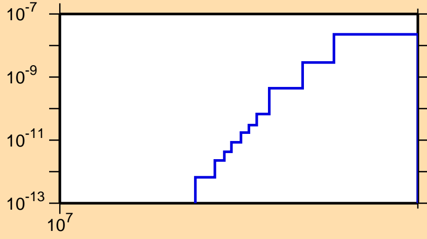
\sigma vs. E for ^{183}\text{Pt}(n,\text{pd})
