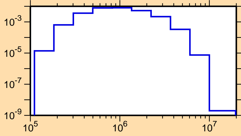
\sigma vs. E for ^{183}\text{Pt}(n,n_4)
