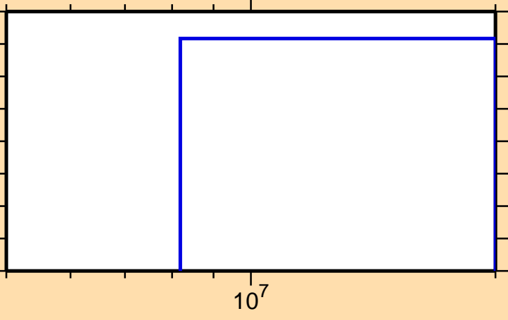
\sigma vs. E for ^{183}\text{Pt}(n,\text{pd})
