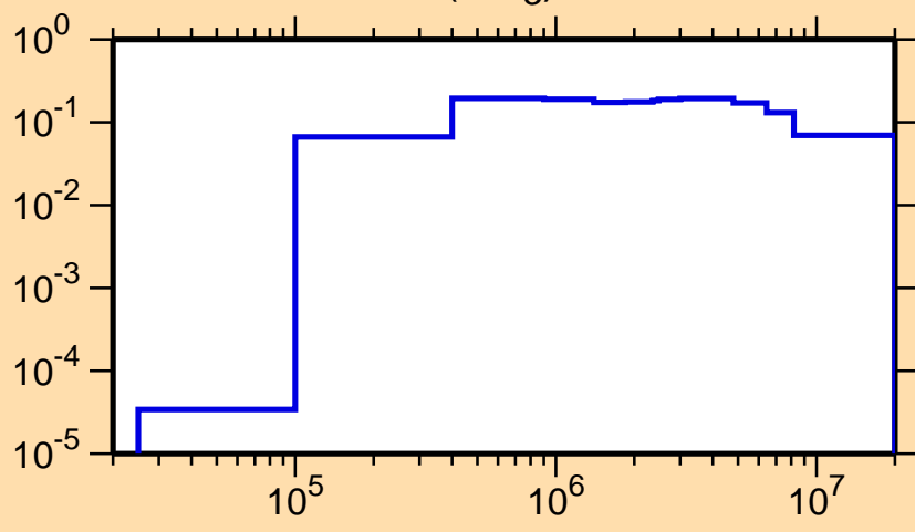
\sigma vs. E for ^{183}\text{Pt}(n,n_3)
