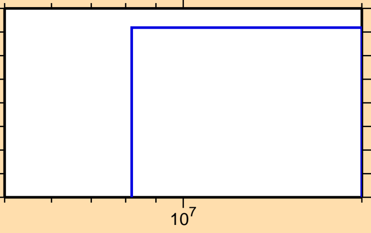
\sigma vs. E for ^{183}\text{Pt}(n,\text{nd})
