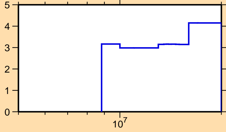
\Delta\sigma/\sigma vs. E for ^{184}\text{Pt}(n,\text{tot.})
