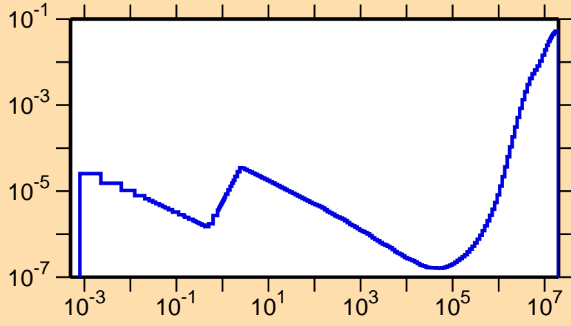
\sigma vs. E for ^{184}\text{Pt}(n,p)
