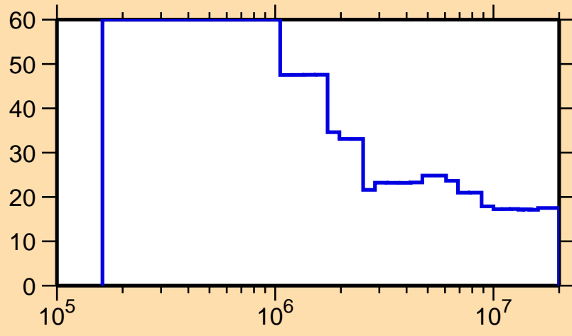
\Delta\sigma/\sigma vs. E for ^{184}\text{Pt}(n,n_1)
