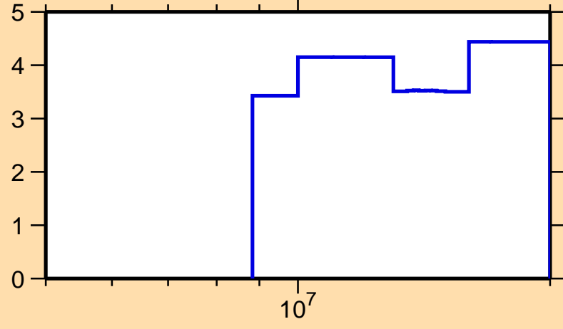
\Delta\sigma/\sigma vs. E for ^{184}\text{Pt}(n,\text{el.})
