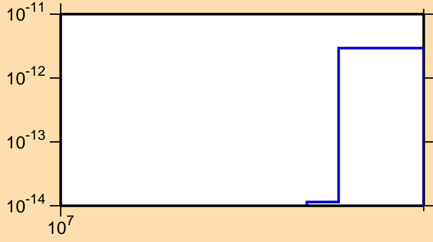
\sigma vs. E for ^{184}\text{Pt}(\text{mt } 34)
