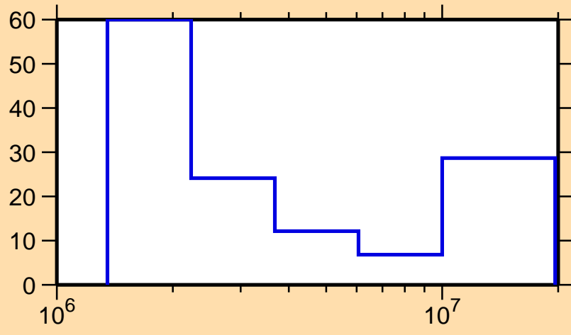
\Delta\sigma/\sigma vs. E for ^{184}\text{Pt}(n,ncont.)
