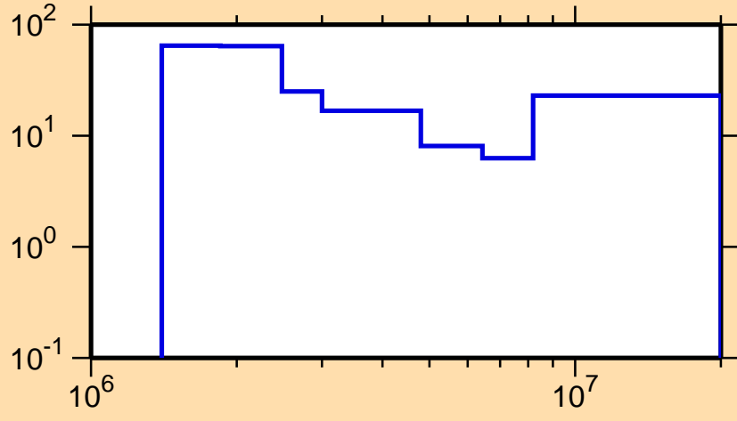
\Delta\sigma/\sigma vs. E for ^{184}\text{Pt}(n,ncont.)
