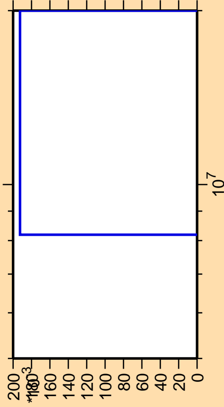
\Delta\sigma/\sigma vs. E for ^{184}\text{Pt}(\text{mt } 34)
