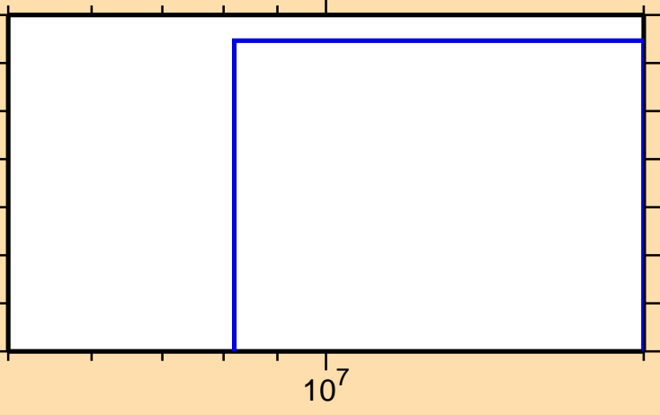
\sigma vs. E for ^{184}\text{Pt}(n,3n)
