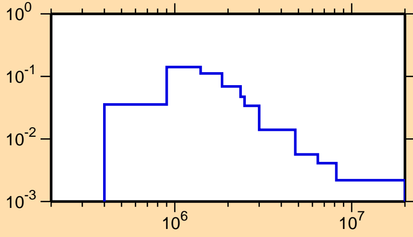
\sigma vs. E for ^{184}\text{Pt}(n,n_4)
