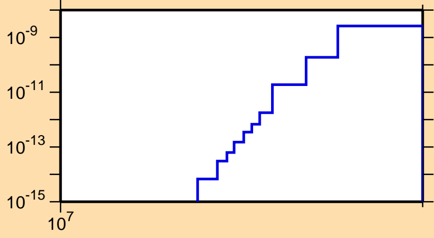
\sigma vs. E for ^{185}\text{Pt}(n,pd)
