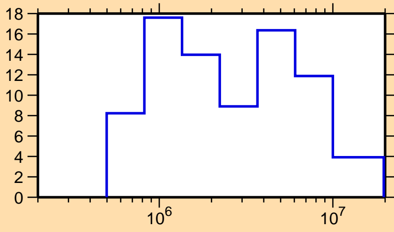
\Delta\sigma/\sigma vs. E for ^{185}\text{Pt}(n, \text{el.})
