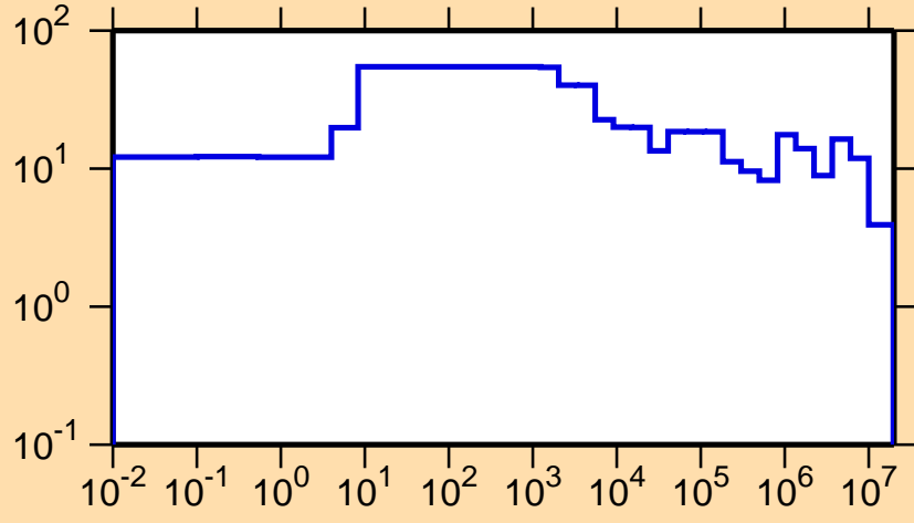
\Delta\sigma/\sigma vs. E for ^{185}\text{Pt}(n,el.)
