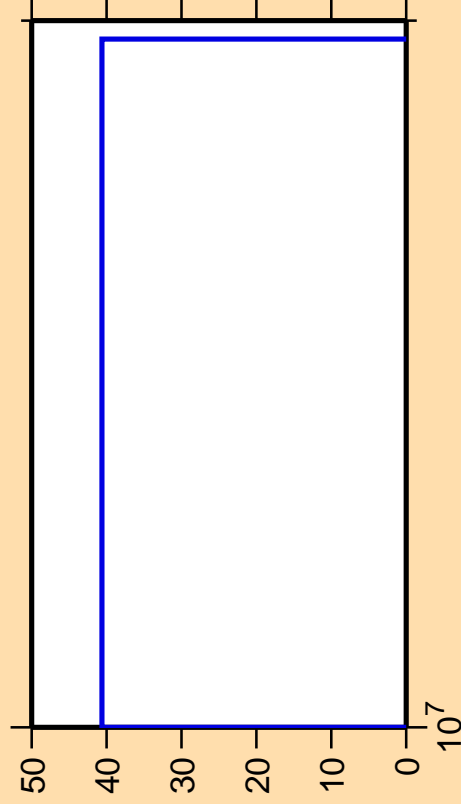
\Delta\sigma/\sigma vs. E for ^{185}\text{Pt} (mt 45)
