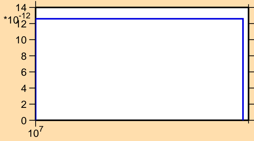
\sigma vs. E for ^{185}\text{Pt} (mt 45)
