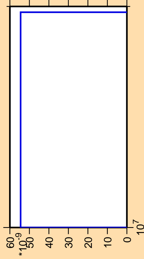
\Delta\sigma/\sigma vs. E for ^{185}\text{Pt} (mt 11)
