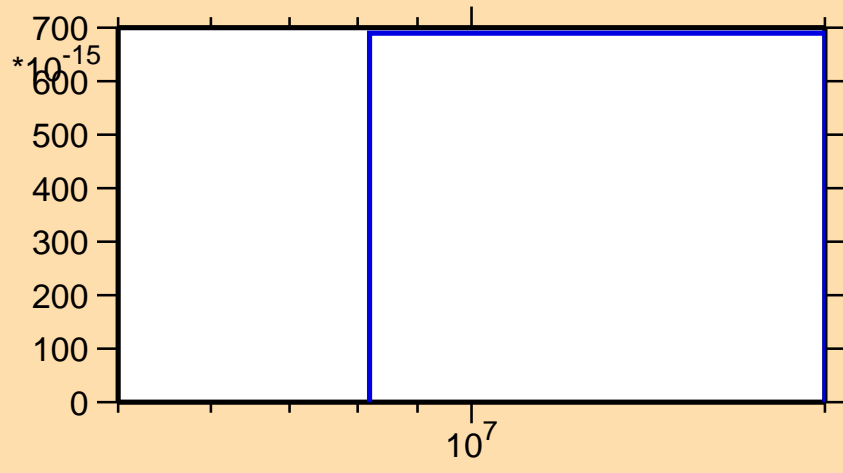
\sigma vs. E for ^{185}\text{Pt}(\text{mt117})
