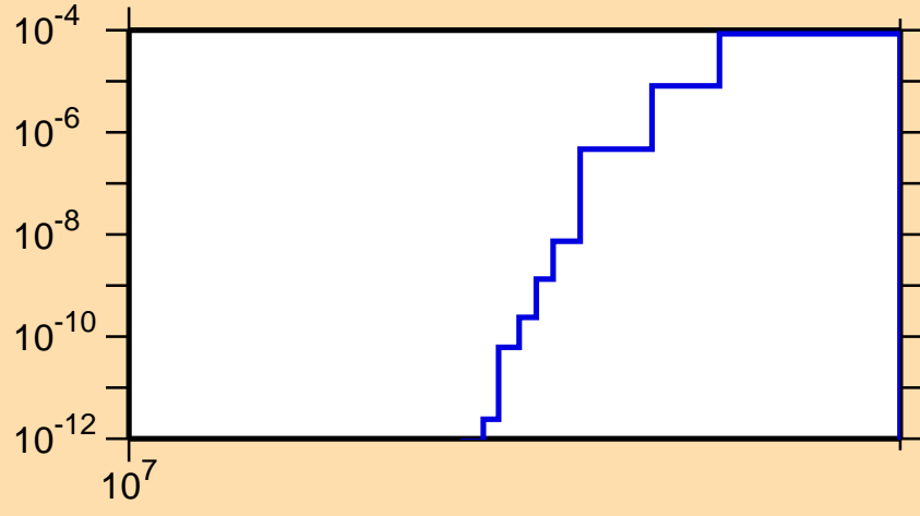
\sigma vs. E for ^{185}\text{Pt}(n,2np)
