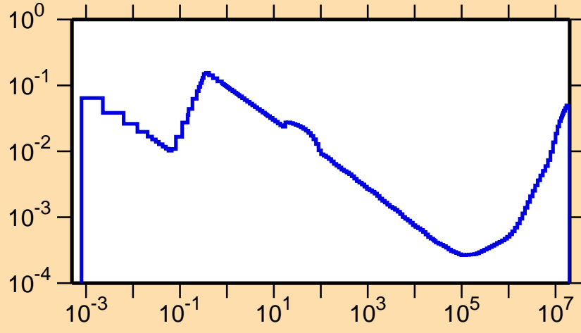
\sigma vs. E for ^{185}\text{Pt}(n,p)
