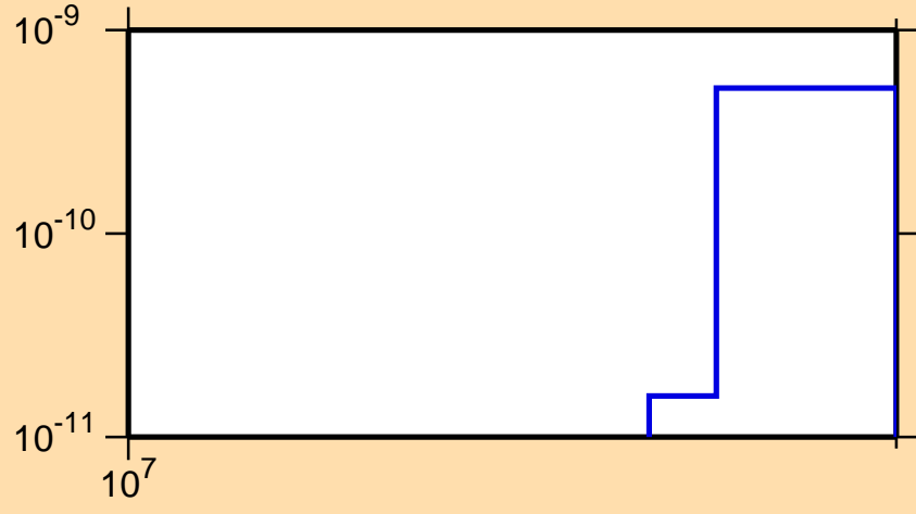
\sigma vs. E for ^{185}\text{Pt}(n,\text{pt})
