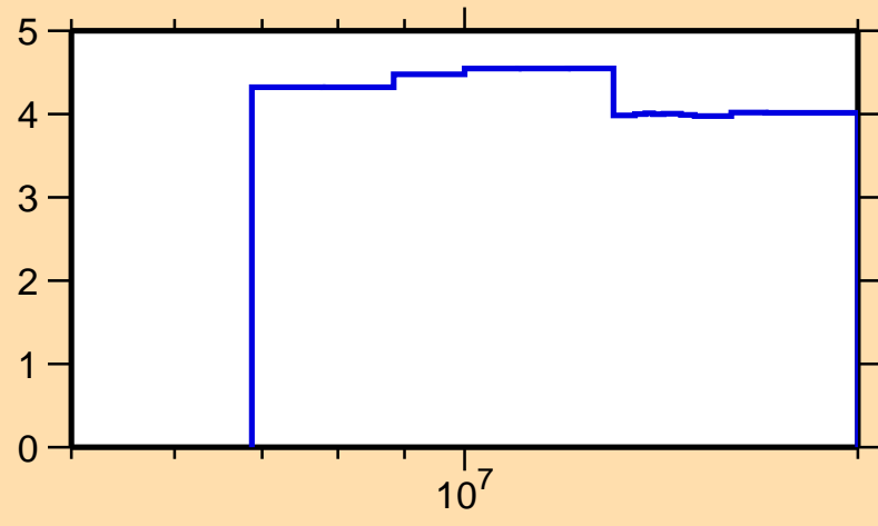
\Delta\sigma/\sigma vs. E for ^{185}\text{Pt}(n,\text{nonel.})
