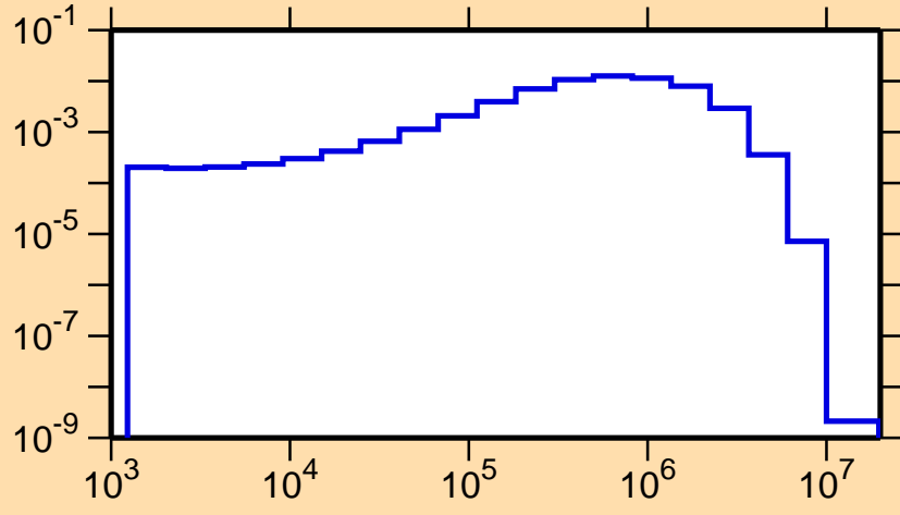
\sigma vs. E for ^{185}\text{Pt}(n,n_1)
