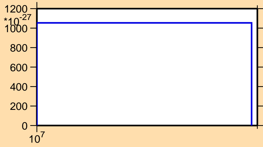
\sigma vs. E for ^{185}\text{Pt} (mt 11)
