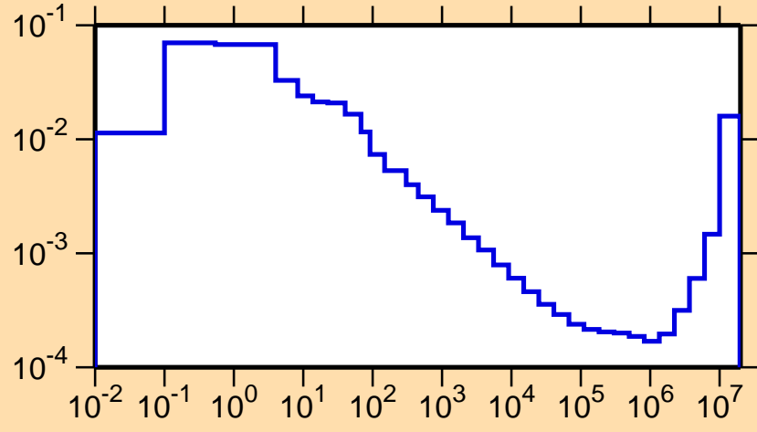
\sigma vs. E for ^{185}\text{Pt}(n,\alpha)
