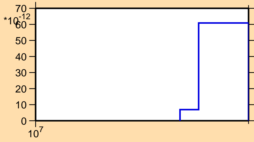
\sigma vs. E for ^{186}\text{Pt}(\text{mt117})
