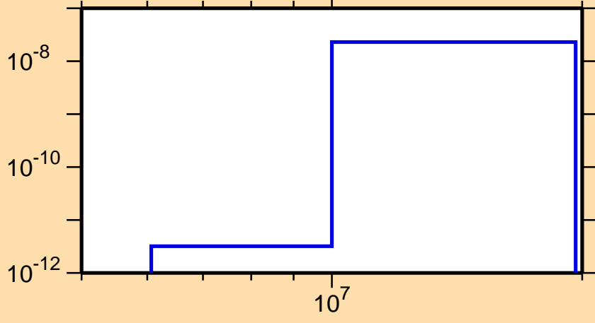
\sigma vs. E for ^{186}\text{Pt}(n,p\alpha)
