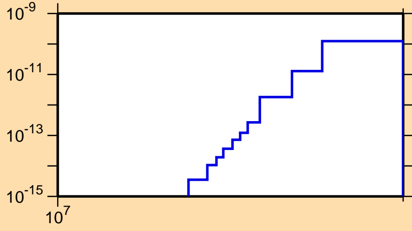
\sigma vs. E for ^{187}\text{Pt}(\text{mt } 45)
