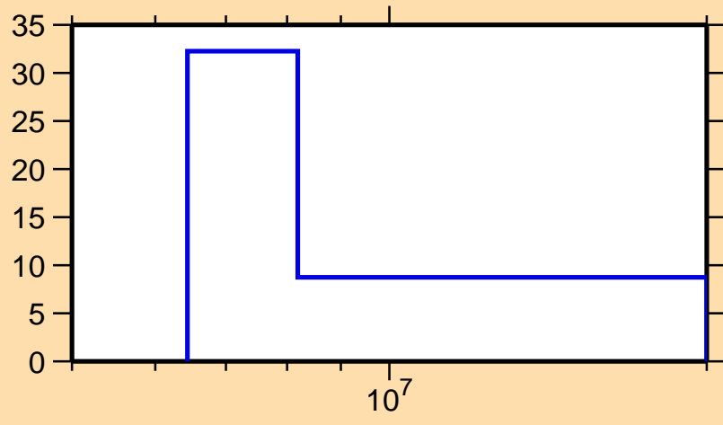
\Delta\sigma/\sigma vs. E for ^{187}\text{Pt}(n,2n)
