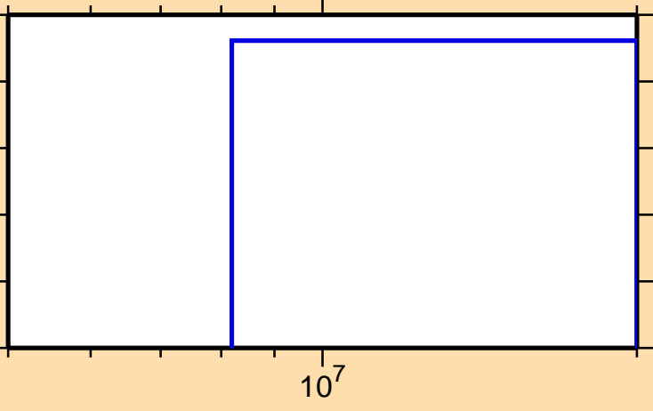
\sigma vs. E for ^{187}\text{Pt}(n,3n\alpha)
