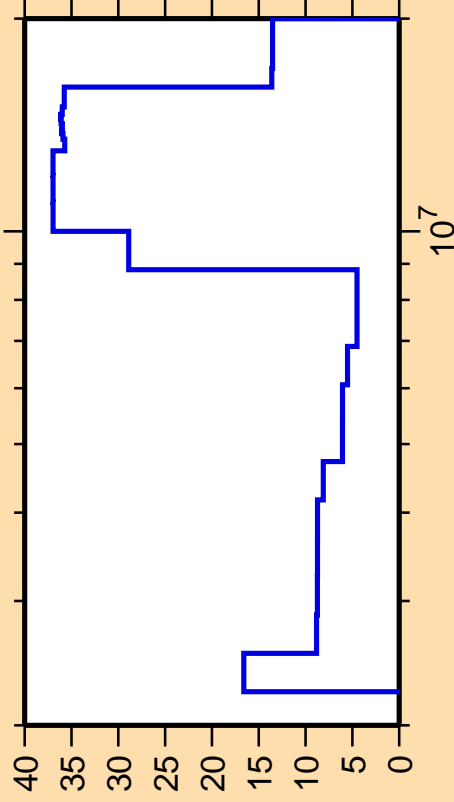
\Delta\sigma/\sigma vs. E for ^{188}\text{Pt}(n,n\text{cont.})
