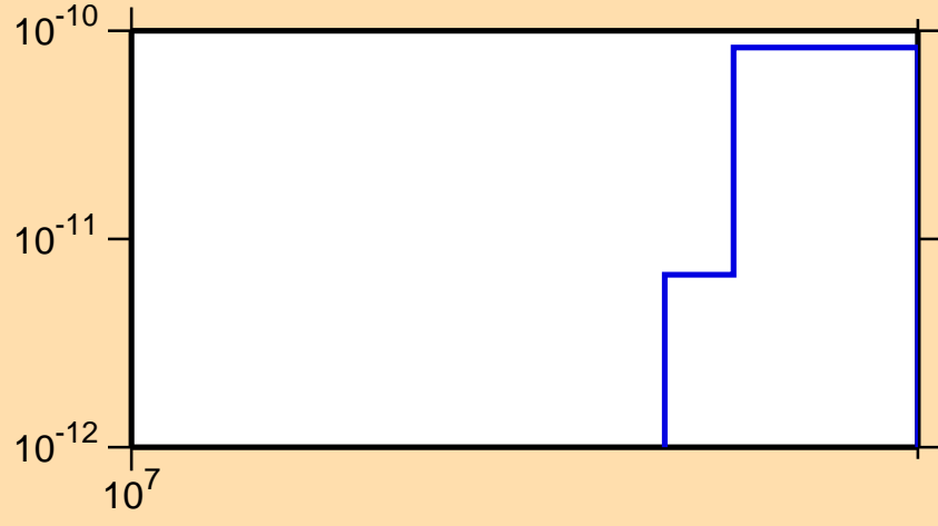
\sigma vs. E for ^{188}\text{Pt}(\text{mt } 45)
