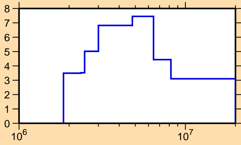
\Delta\sigma/\sigma vs. E for ^{188}\text{Pt}(n, el.)
