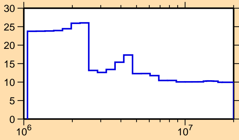
\Delta\sigma/\sigma vs. E for ^{189}\text{Pt}(n,n_1)
