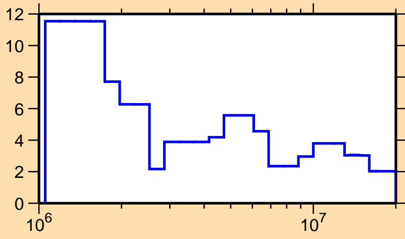
\Delta\sigma/\sigma vs. E for ^{189}\text{Pt}(n, el.)
