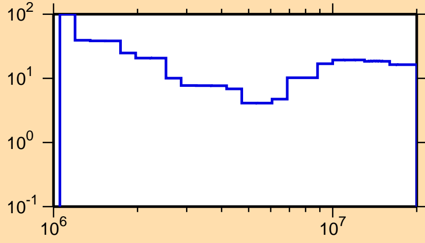
\Delta\sigma/\sigma vs. E for ^{189}\text{Pt}(n,n\text{cont.})
