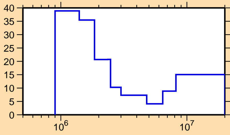
\Delta\sigma/\sigma vs. E for ^{189}\text{Pt}(n,ncont.)
