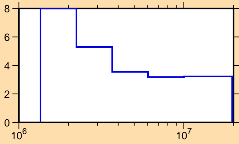
\Delta\sigma/\sigma vs. E for ^{190}\text{Pt}(n,\text{nonel.})
