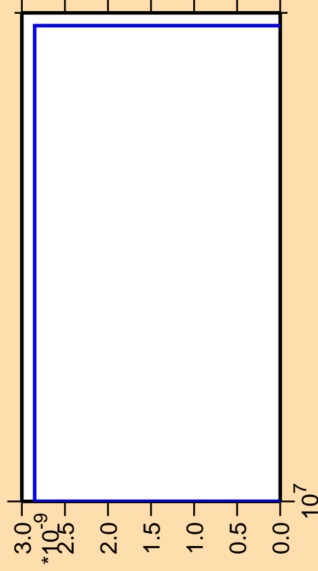
\Delta\sigma/\sigma vs. E for ^{190}\text{Pt} (mt 11)
