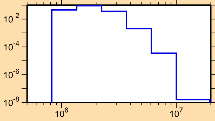
\sigma vs. E for ^{190}\text{Pt}(n,n_4)
