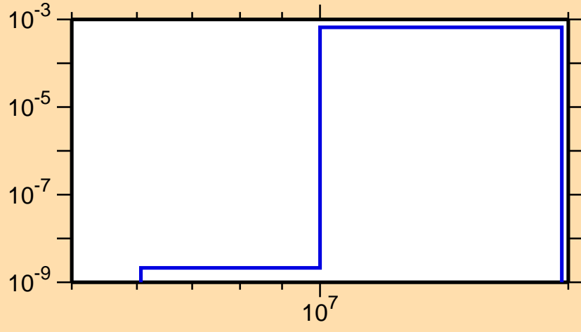
\sigma vs. E for ^{190}\text{Pt}(n,d)
