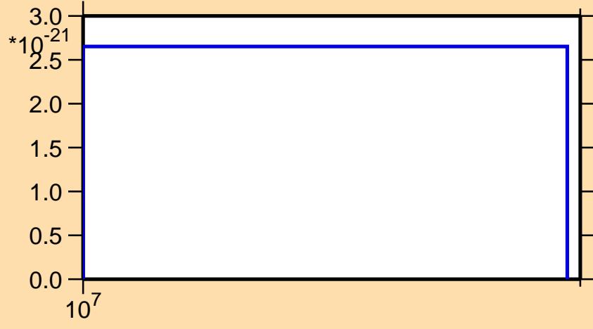
\sigma vs. E for ^{190}\text{Pt} (mt 11)
